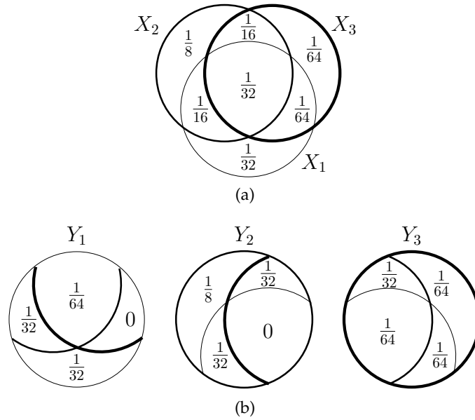
Figure 4.6: Disentangling sets
