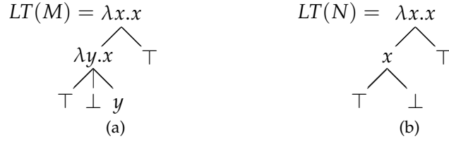
Figure 5.2: Lévy-Longo trees of M and N .
