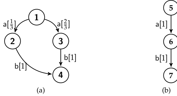
Figure 4.3: Two bisimilar probabilistic systems.
