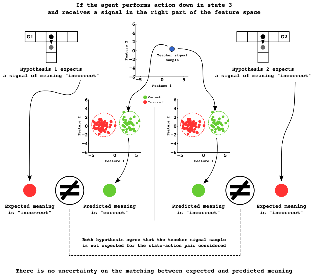
Figure 5.11: Matching between expected labels and the prediction of a teaching signal sampled on the right side of the feature space for the two hypothesis if the agent performs action down in state 3 and the two hypothesis currently have a symmetric interpretation of the signals (see Figure 5.2). Both hypotheses agree that the label associated to a signal on the right side of the feature space does not match with the label predicted given the frame and the state-action pair considered. Therefore there is no uncertainty associated to this state-action pair and the agent should not select action down.
