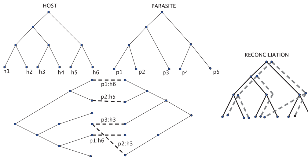
Figure 1.4: A schematic representation of a phylogenetic reconciliation
