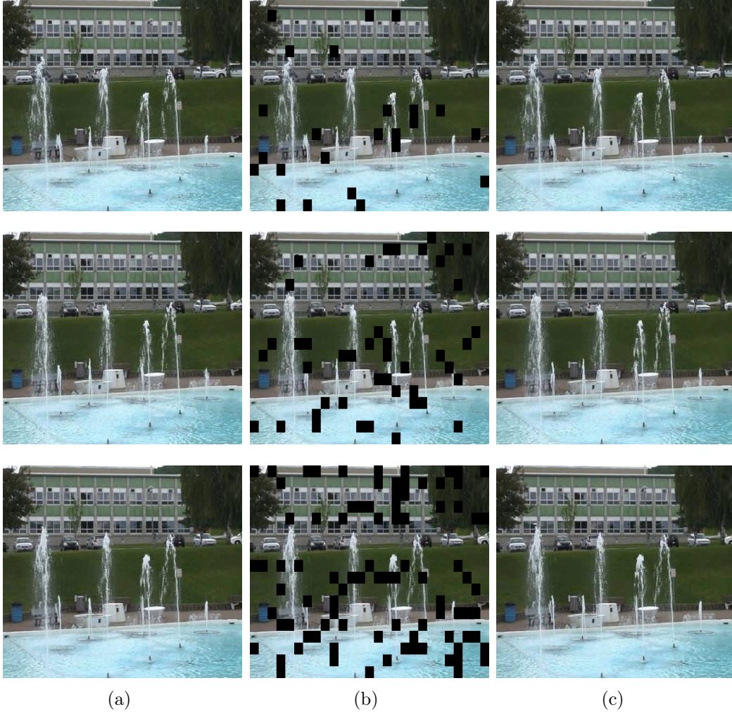
Figure 5.13: Error concealment results of the sequence fountain01. Three frames of the scene with three different loss rate of 16 \times 16 blocks. From top to bottom: respectively 5%, 10% and 20% of blocks are lost. (a) Input frames. (b) Frames with the missing blocks. (c) Inpainting results using the proposed approach.
