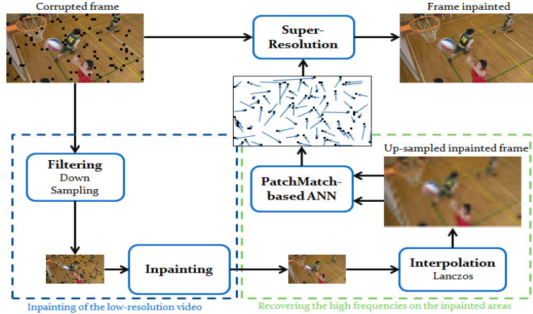
Figure 3.4: Two-steps multi-resolution extension. A low resolution version of the input video is first inpainted, and the details of the inpainted areas are retrieved using an ANN-based super-resolution technique (ANN stands for Approximate Nearest Neighbors).
