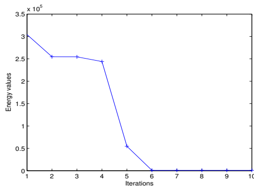
Figure 5.7: Energy convergence.
