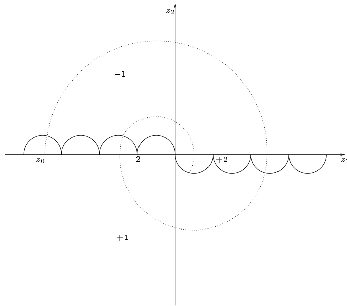
Figure 4.2: Switching curve for the harmonic oscillator (solid line) and time-optimal solution for the initial condition z_0 (dotted line), which presents 4 switches
