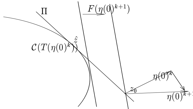
Figure 4.3: Description of one step of Neustadt's algorithm
