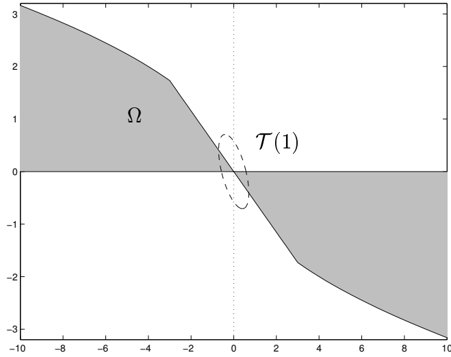
Figure 3.2: The regions \Omega (shaded) and \mathcal{T}(1) for the double integrator in the (x_1, x_2) state-space. The corner in the boundary at (-3, \sqrt{3}) in the boundary of the \Omega region is due to the transition from the boundary defined by V(x, \epsilon) = \bar{V}(\epsilon) to the boundary defined by \epsilon = 1
