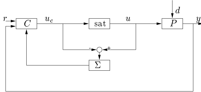
Figure 1.1: Canonical form of anti-windup schemes
