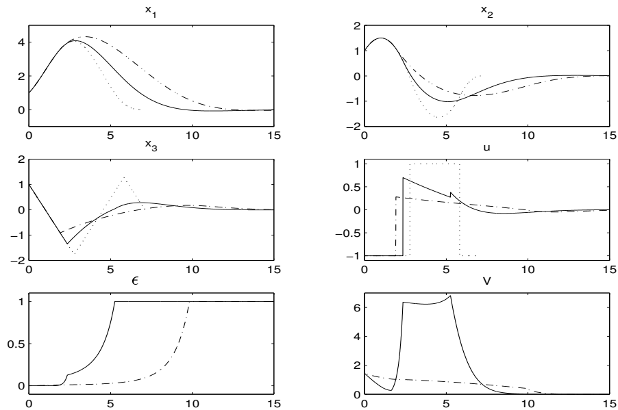
Figure 3.4: Control of the third order integrator: time optimal method (dotted), Lin-Megretski's method with k = \frac{1}{\epsilon} (dash-dotted) and our method (solid) ( (x_{10}, x_{20}, x_{30}) = (1, 1, 1) )
