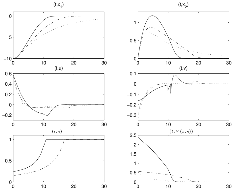
Figure 3.6: Solution of the controlled double integrator with amplitude and rate constraint on the control variable ( u_{max} = 1 and v_{max} = 1 ). The application of a low-gain control law without gain-scheduling (dotted line) is compared to a control law with explicit (dash-dotted line) and implicit gain-scheduling (solid line)
