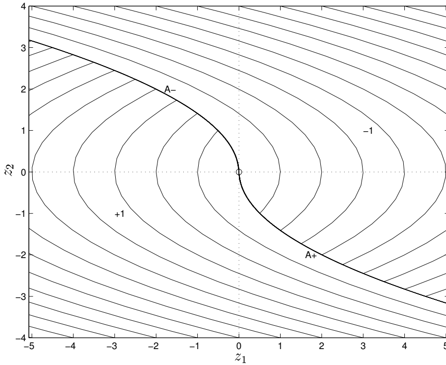
Figure 4.1: Phase plane of the time-optimal control of the double integrator
