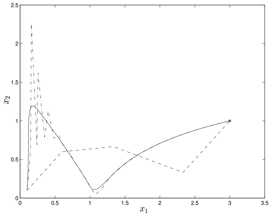
Figure 4.8: Phase plane evolution of the algorithm: (solid line) Runge-Kutta's method with a time-scale separation; (dash-dotted) Euler with time-scale separation; (dashed) Euler without time-scale separation.
