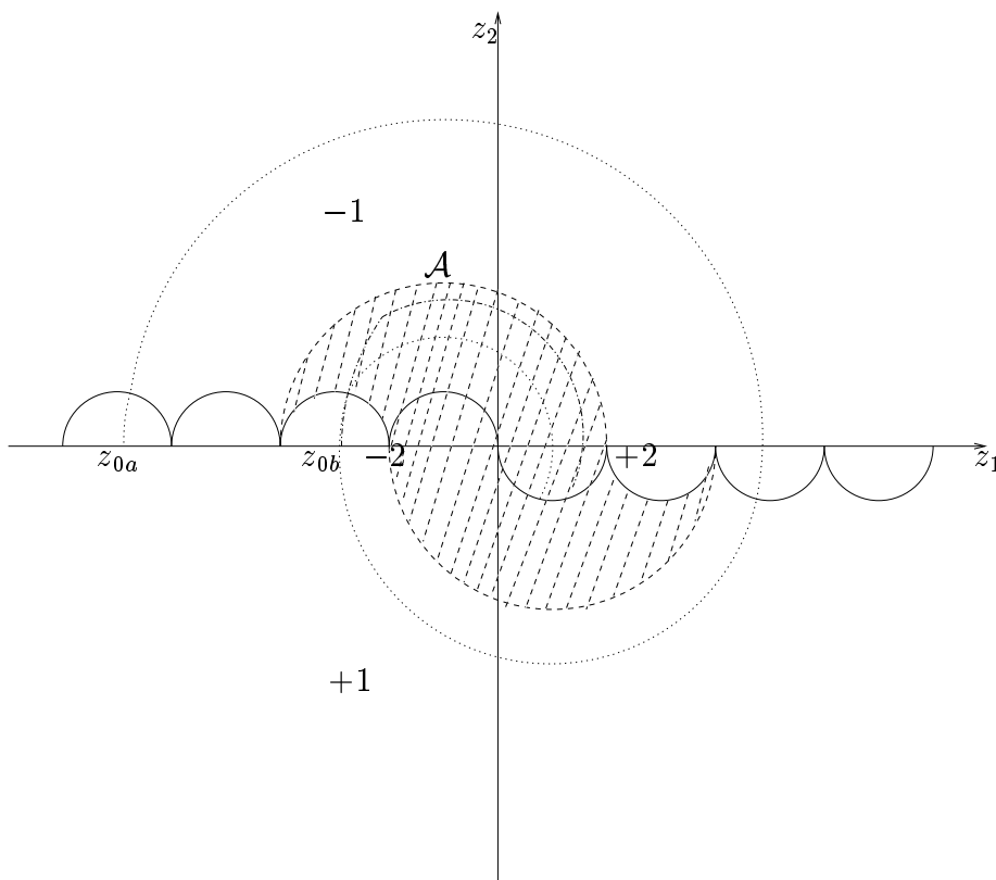
Figure 4.10: Phase plane of the time-optimal control of the harmonic oscillator: (solid line) switching curve; (dotted line) the time-optimal solution initiating at z_{0a} and going through z_{0b} ; (dash-dotted line) a bang-bang solution with two switches starting at z_{0b}
