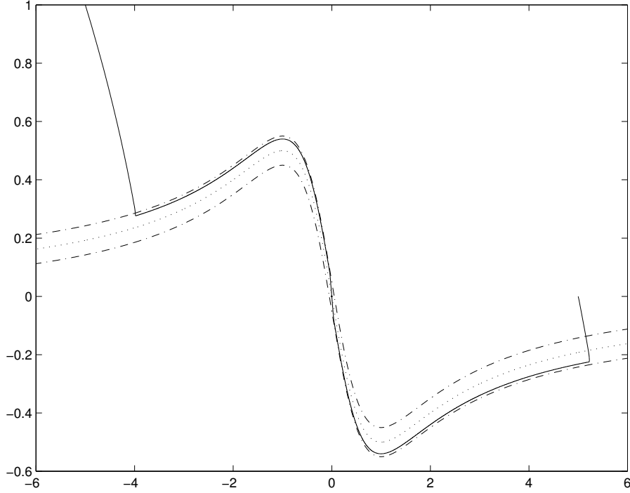
Figure 2.1: Phase plane of the slow control of example (2.18) with x_0 = (-5 \ 1)^T and x_0 = (5 \ 0)^T as initial conditions (solid line). The manifold x_2 + \frac{x_1}{1+x_1^2} = 0 is illustrated (dotted line), as well as the invariant interval around it (between the dash-dotted lines)
