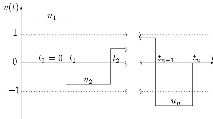
Figure 4.4: Control sequence
