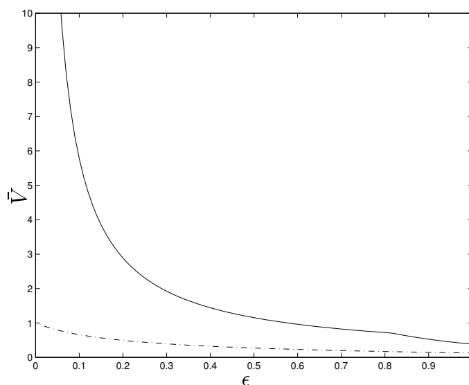
Figure 3.5: Evolution of \bar{V}(\epsilon) for the explicit (dash-dotted line) and the implicit schedulings (solid line)
