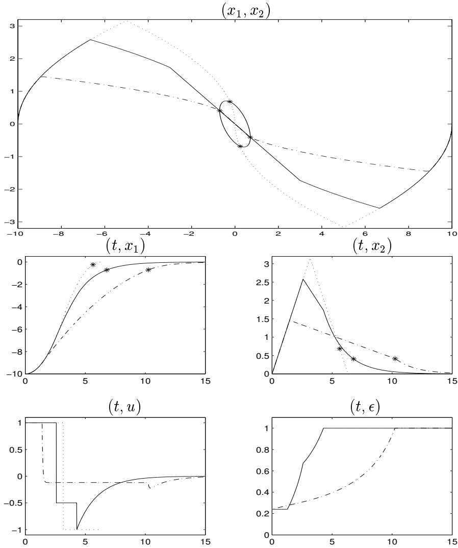
Figure 3.3: Phase plane and time evolutions for the double integrator with initial condition (x_{10}, x_{20}) = (-10, 0) : time optimal method (dotted), explicit controller of Megretski (1996) with k = \frac{1}{\epsilon} (dash-dotted) and proposed implicit controller (solid). Stars indicate the time instants or the points in state-space at which the solutions reach \mathcal{T}(1) .
