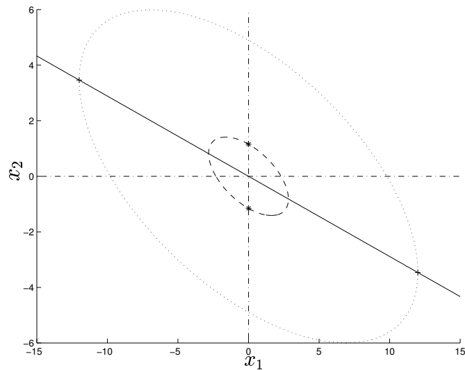
Figure 3.1: The manifold b^T P(0.5)x = 0 is drawn (solid line). Both the high-and-low-gain method and the invariance checking method force the solution to follow this manifold. This can be achieved in the dashed level set for the high-and-low gain method because |b^T P(0.5)x| = 1 at the stars. On the other hand the control that ensures invariance of b^T P(0.5)x = 0 reaches 1 at the +, and define the admissible level set for the invariance checking method (dotted ellipse). The rate of convergence corresponding to \epsilon = 0.5 can be achieved in a much large region
