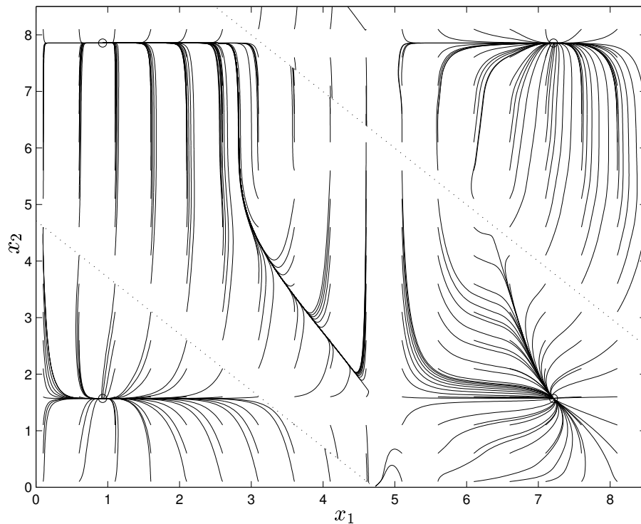
Figure 4.11: Phase plane of the evolution of the continuous algorithm with z_0 = (1 \ 1)^T . Four equilibria, including the time optimal solution x = (0.9305 \ 1.5709)^T , are represented. They are all attractive and their region of attraction is apparent on the figure
