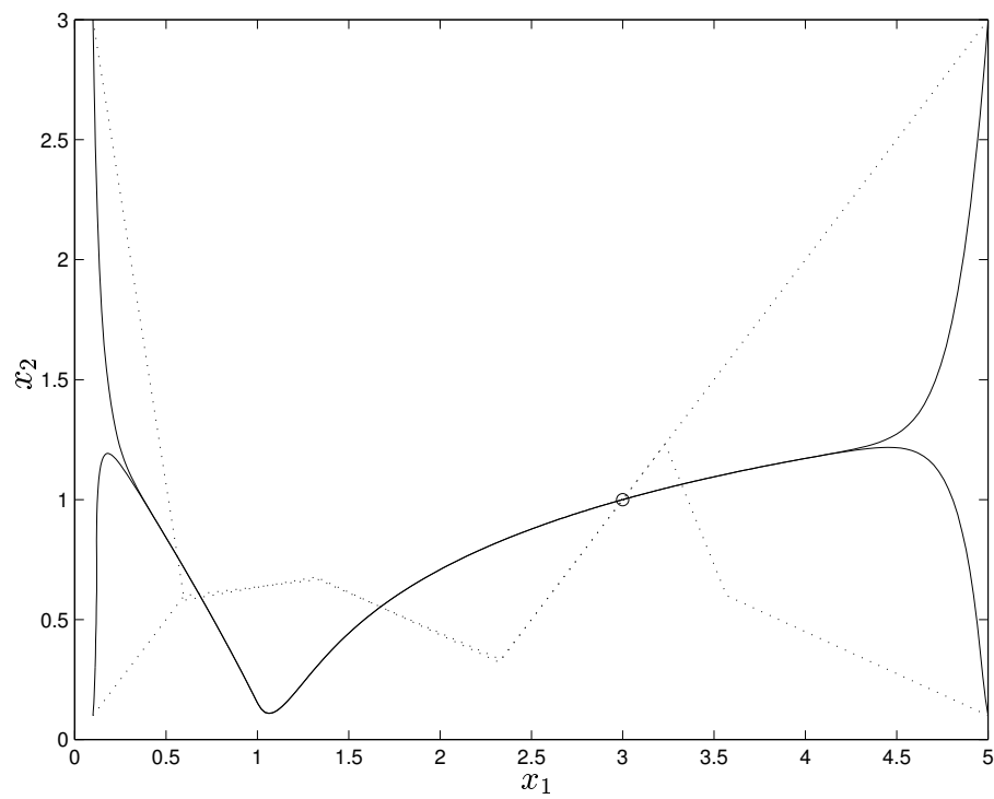
Figure 4.9: Phase plane evolution of the algorithm: (solid line) Runge-Kutta's method with a time-scale separation; (dotted line) Euler without time-scale separation.
