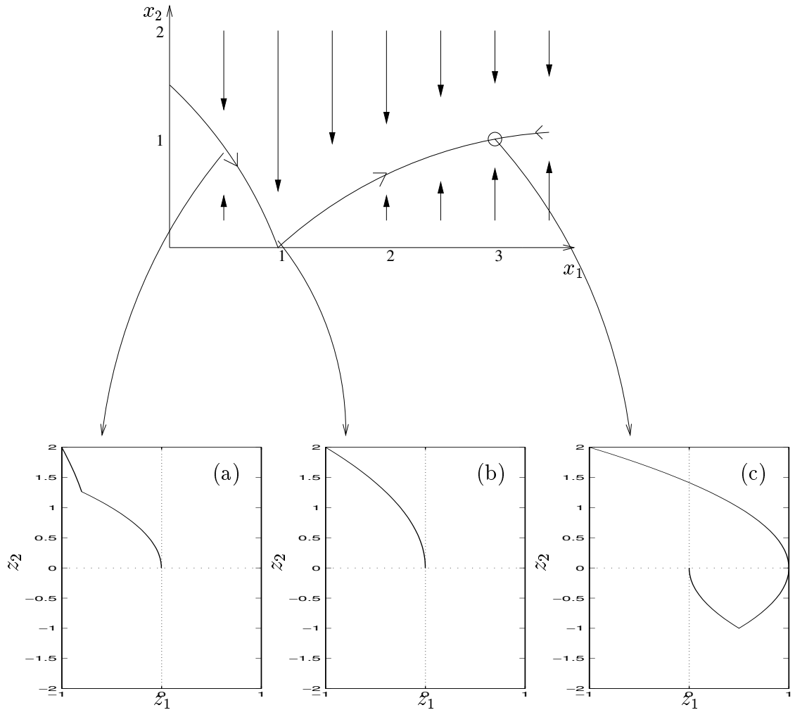
Figure 4.6: Top: Phase portrait of (4.13) for \epsilon \rightarrow 0 . Bottom: Evolution of the solution (z_1(t), z_2(t)) along the application of the algorithm: (a) \{x, u\} = \{(0.1228, 1.2649)^T, (-6, -1)^T\} ; (b) \{x, u\} = \{(1, 0)^T, (-2, 0)^T\} (c) \{\bar{x}, \bar{u}\} = \{(3, 1)^T, (-1, 1)^T\} . Figure (b) represents the singularity, where the origin is reached without switching, and Figure (c) represents the time-optimal solution.
