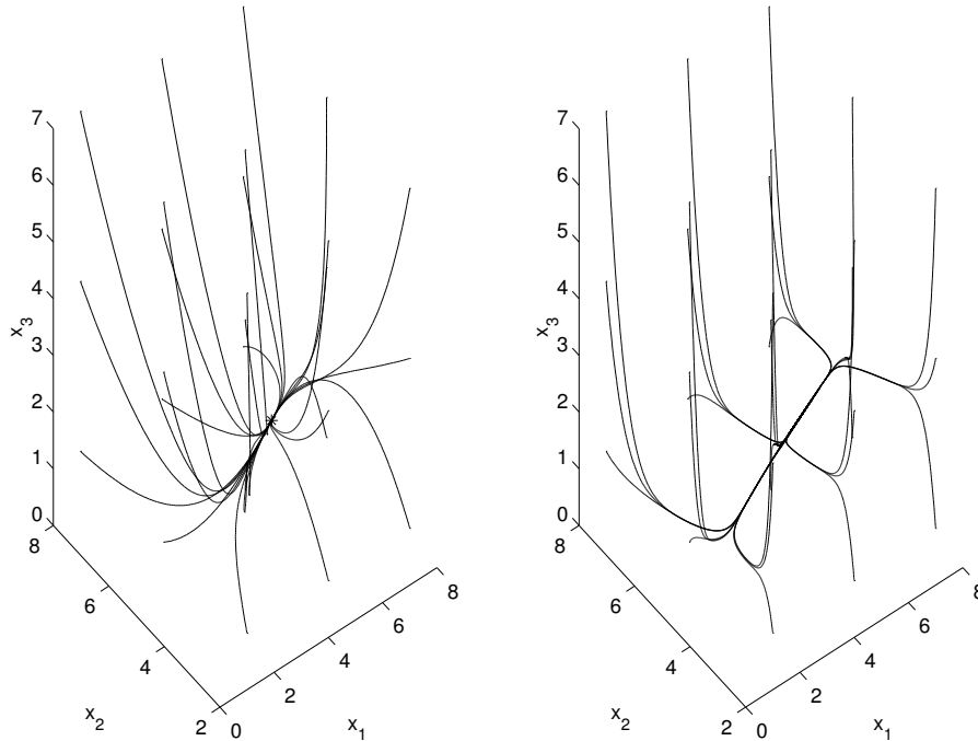
Figure 4.5: Simulations of (4.12) for the triple integrator \frac{d^3 y}{dt^3} = u . The initial condition in the state-space is y(0) = \dot{y}(0) = \ddot{y}(0) = 2 . The time-scale separation is ensured with, respectively, \epsilon_1 = 2\epsilon_2 = 4\epsilon_3 = 1 (left) and \epsilon_1 = 10\epsilon_2 = 100\epsilon_3 = 1 (right). The strong time-scales separation appears on the right, while it is clear that convergence takes place on the left, even with a weak separation.
