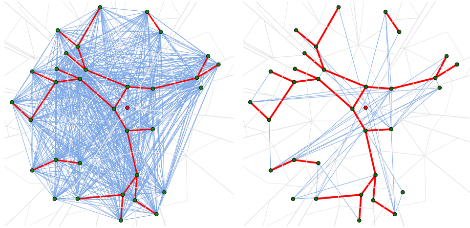
Figure 7.6: Left: In the case of unknown doublets and triplets, naively, all possible pairs of points have to be considered. Right: Our geometric constraints are able to remove most of the false connections. The weakly visible unfolding geometry is shown only for illustration. It is still unknown at this point of our algorithm.
