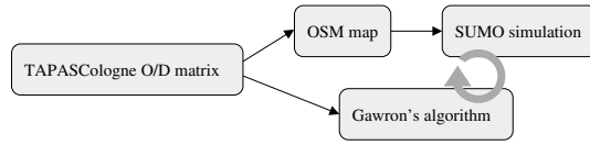
Figure 2.2: Cologne mobility dataset generation workflow.
