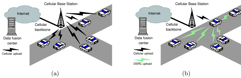
Figure 3.12: FCD upload scenarios. (a) Traditional via the cellular infrastructure. (b) Offloaded through V2V transfers.
