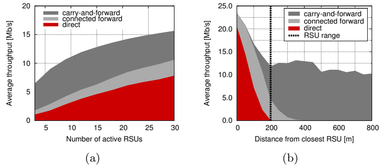
Figure 3.5: Cooperative download at low-penetration regime. (a) Transfer paradigm split-up of the average per-downloader throughput. (b) Average per-downloader throughput versus the distance between the downloader and the closest RSU.
