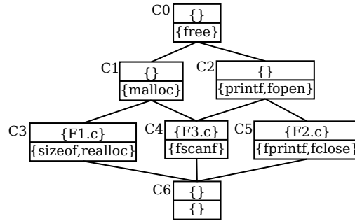
Figure 6.2: Lattice of concepts for the data set in Table 6.3
