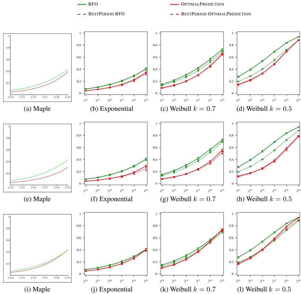
Figure 2.3: Waste (y-axis) for the different heuristics as a function of the platform size (x-axis), with p = 0.4 , r = 0.7 , C_p = C (first row), C_p = 0.1C (second row), or C_p = 2C (third row) and with a trace of false predictions parameterized by a distribution identical to the distribution of the failure trace.
