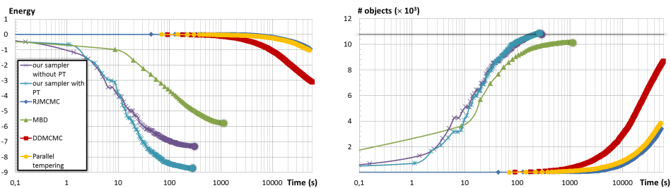
Figure 8: Performances of various samplers. The left graph describes the energy decrease over time from the bird image presented in Fig. 7 (the colored dots correspond to algorithm convergence). Note that time is represented using a logarithmic scale, and that the slow convergence of RJMCMC [Gre95], DDMCMC [TZ02], and parallel tempering [ED05] algorithms is not displayed on the graph. The right graph shows the evolution of the number of objects during the sampling. Contrary to the other samplers, the number of objects found by our sampler with and without space-partitioning tree (PT) is very close to the ground truth (black line).
