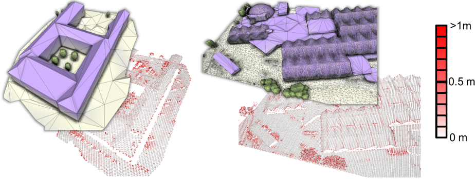
Figure 28: Building reconstruction - ( top ) obtained 3D-model and ( bottom ) input cloud ( 2\text{pts}/\text{m}^2 ) with the points colored according to their distance to the 3D-model. The high errors correspond to points from trees (the points of a tree do not obviously describe a perfect ellipsoidal shape) and from small urban components such as cars or roof superstructures. The left building is highly regular, the roof being entirely explained by planar primitives. The right building is more complex as it contains atypical roof forms, ie the undulating roof sections and the spherical dome. A hybrid surface is particularly relevant in such a case.
