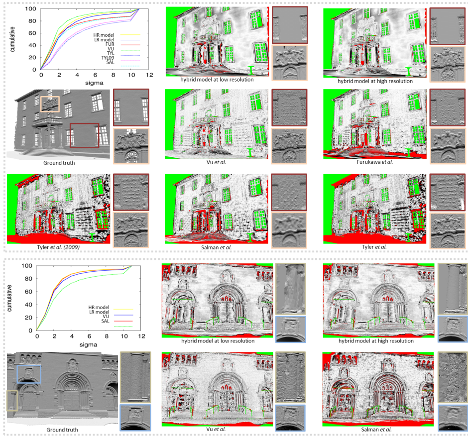
Figure 25: Accuracy evaluation on Entry-P10 (top) and Herz-Jesu-P25 (bottom). The cumulative error histograms are measured with respect to the standard deviation \Sigma of the ground truth accuracy [SVHVG+08]. The error maps of the different models are established with respect to the ground truth (white=low, black=high, red=off-the-scale). Our high resolution hybrid models obtain the first and second best accuracies for Herz-Jesu-P25 and Entry-P10 respectively.
