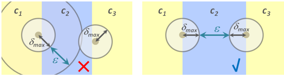
Figure 5: Independence of cells. On the left case, the width of the cell c_2 is not large enough to ensure the independence of the cells c_1 and c_3 : the two grey points in c_1 and c_3 cannot be perturbed at the same time. On the right case, the cells c_1 and c_3 are independent as Eq. 14 is satisfied.
