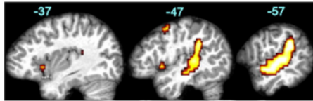
2D plot(s) of the detections
