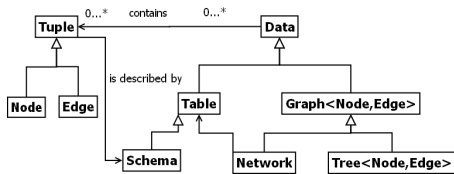
Figure 2: Class diagram of the Obvious data model
