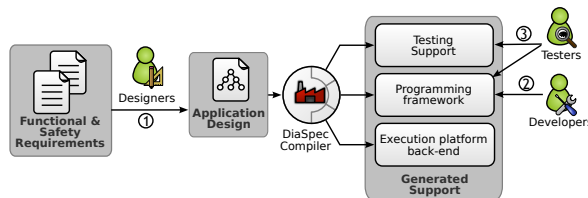
Figure 4: The DiaSuite tool-based methodology
