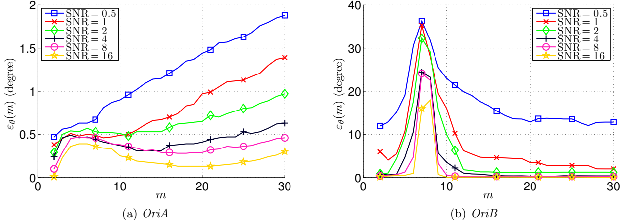
Figure 11: The average difference in the estimated principal direction \varepsilon_{\theta}(m) between the noise-free image and the noisy images of different SNR of the two datasets OriA (a) and OriB (b). A small value of \varepsilon_{\theta}(m) means that the principal direction estimated by the generic R -transform is very stable under noise perturbation.
