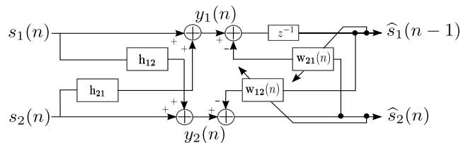
Figure 1: Mixing model (left) and separation structure (right). The introduced delay arbitrarily fixed in the separation structure is justified by implementation considerations.
