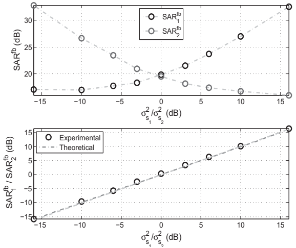
Figure 7: Frequency average SAR_i^{fb} obtained on channel 1 and 2 when \alpha = 0 for different values of \sigma_{s_1}^2/\sigma_{s_2}^2 .
