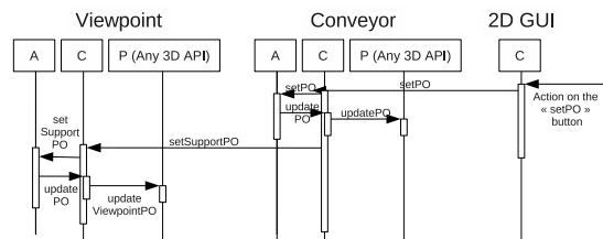
Figure 16: Delegating navigation to the abstraction of a viewpoint
