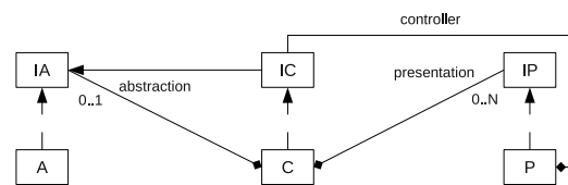
Figure 6: The PAC model with interfaces between facets
