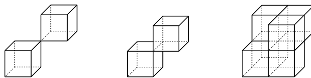
Fig. 2. The forbidden configurations
