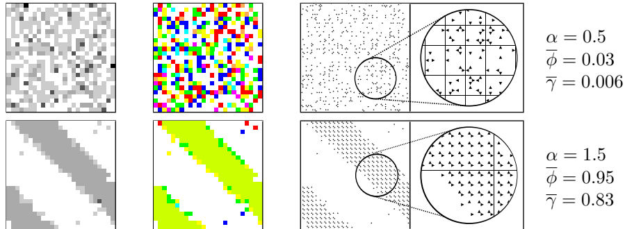
Figure 4: Observation of a random distribution (top) and the diagonal stripe (bottom) pattern. The visualisations are particle density (left), flux (middle) and channels (right), for L = 25 , t = 1000 , \rho = 0.2 .
