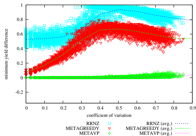
Figure 32: Difference in Achieved Minimum Yield from METAHVP vs Coefficient of Variation on problem instances with 64 hosts, 500 services, memory slack = 0.7
