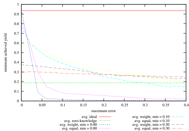
Figure 50: Achieved Minimum Yield from Baseline vs Maximum Specified Error on problem instances with 64 hosts, 250 services, memory slack = 0.8, coefficient of variation = 0.5; values given are averages over successful instances.
