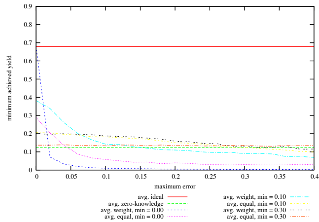
Figure 63: Achieved Minimum Yield from Baseline vs Maximum Specified Error on problem instances with 64 hosts, 500 services, memory slack = 0.2, coefficient of variation = 1.0; values given are averages over successful instances.
