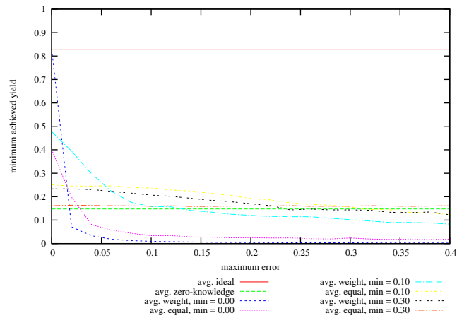
Figure 65: Achieved Minimum Yield from Baseline vs Maximum Specified Error on problem instances with 64 hosts, 500 services, memory slack = 0.6, coefficient of variation = 1.0; values given are averages over successful instances.
