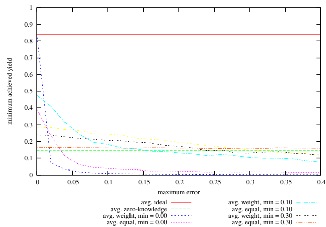
Figure 66: Achieved Minimum Yield from Baseline vs Maximum Specified Error on problem instances with 64 hosts, 500 services, memory slack = 0.8, coefficient of variation = 1.0; values given are averages over successful instances.
