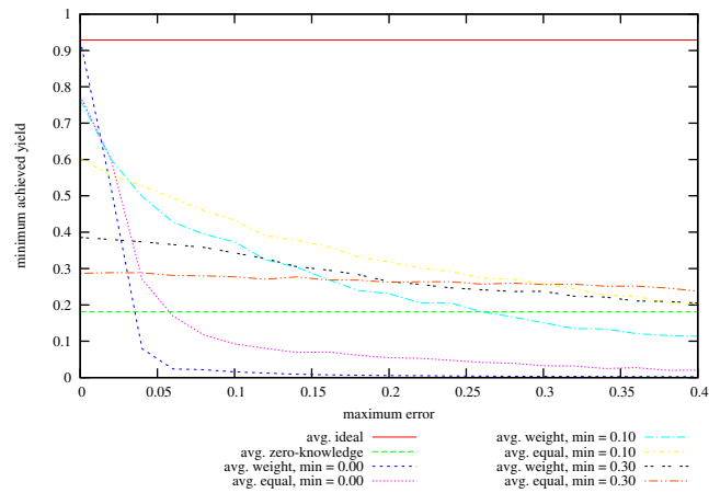
Figure 49: Achieved Minimum Yield from Baseline vs Maximum Specified Error on problem instances with 64 hosts, 250 services, memory slack = 0.6, coefficient of variation = 0.5; values given are averages over successful instances.
