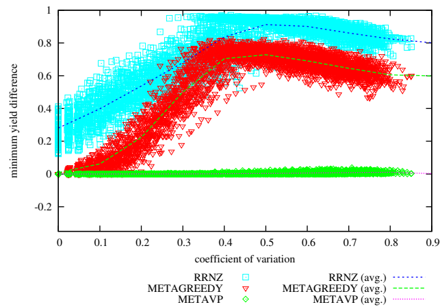
Figure 25: Difference in Achieved Minimum Yield from METAHVP vs Coefficient of Variation on problem instances with 64 hosts, 250 services, memory slack = 0.9
