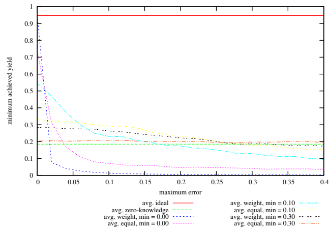
Figure 59: Achieved Minimum Yield from Baseline vs Maximum Specified Error on problem instances with 64 hosts, 500 services, memory slack = 0.2, coefficient of variation = 0.5; values given are averages over successful instances.
