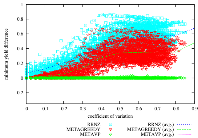
Figure 14: Difference in Achieved Minimum Yield from METAHVP vs Coefficient of Variation on problem instances with 64 hosts, 100 services, memory slack = 0.7
