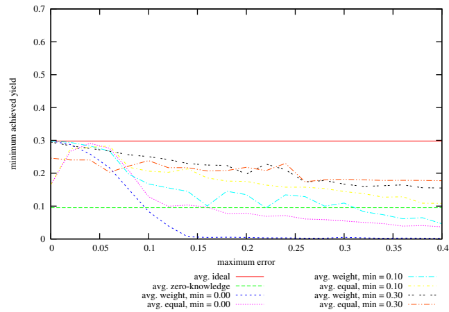
Figure 37: Achieved Minimum Yield from Baseline vs Maximum Specified Error on problem instances with 64 hosts, 100 services, memory slack = 0.4, coefficient of variation = 0.5; values given are averages over successful instances.
