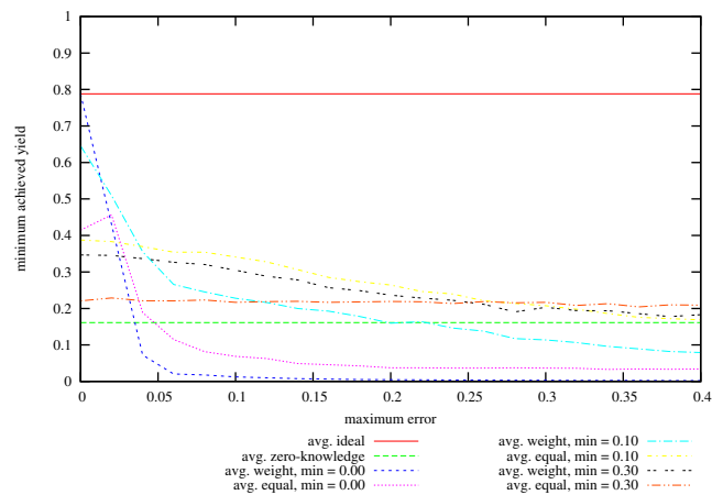
Figure 52: Achieved Minimum Yield from Baseline vs Maximum Specified Error on problem instances with 64 hosts, 250 services, memory slack = 0.4, coefficient of variation = 1.0; values given are averages over successful instances.
