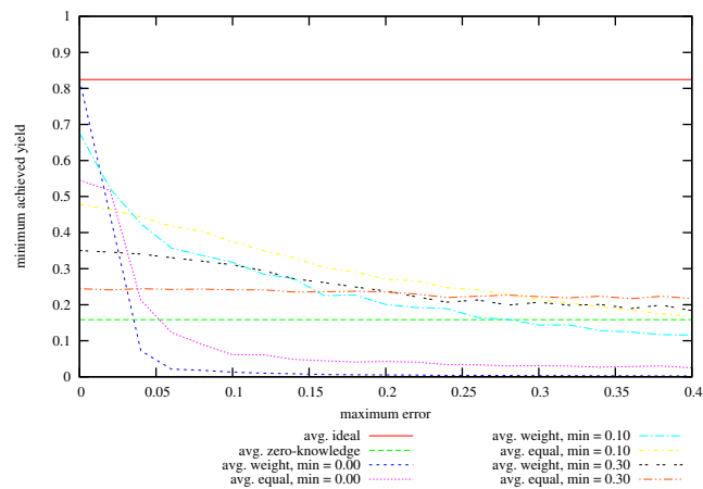
Figure 54: Achieved Minimum Yield from Baseline vs Maximum Specified Error on problem instances with 64 hosts, 250 services, memory slack = 0.8, coefficient of variation = 1.0; values given are averages over successful instances.
