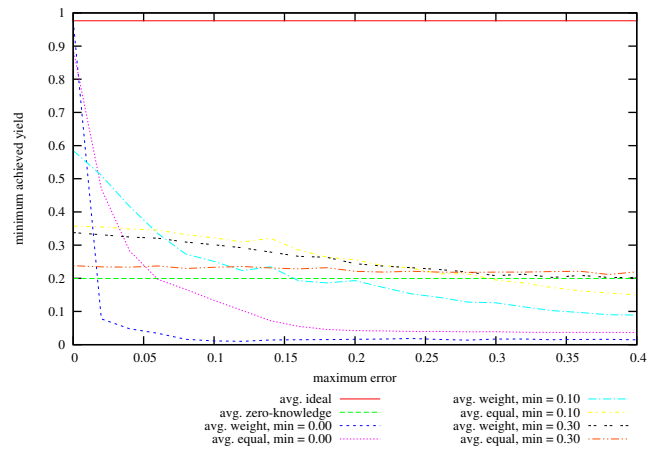
Figure 55: Achieved Minimum Yield from Baseline vs Maximum Specified Error on problem instances with 64 hosts, 500 services, memory slack = 0.2, coefficient of variation = 0.0; values given are averages over successful instances.
