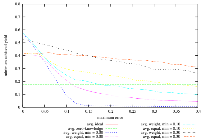
Figure 41: Achieved Minimum Yield from Baseline vs Maximum Specified Error on problem instances with 64 hosts, 100 services, memory slack = 0.6, coefficient of variation = 1.0; values given are averages over successful instances.
