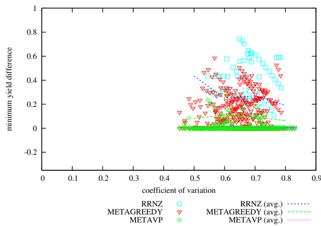
Figure 11: Difference in Achieved Minimum Yield from METAHVP vs Coefficient of Variation on problem instances with 64 hosts, 100 services, memory slack = 0.4
