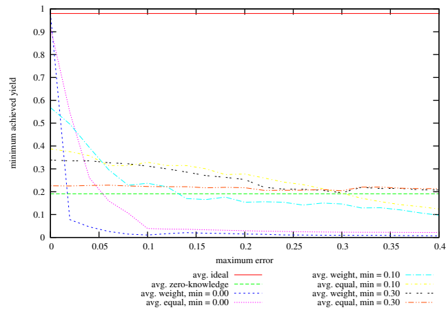
Figure 57: Achieved Minimum Yield from Baseline vs Maximum Specified Error on problem instances with 64 hosts, 500 services, memory slack = 0.6, coefficient of variation = 0.0; values given are averages over successful instances.
