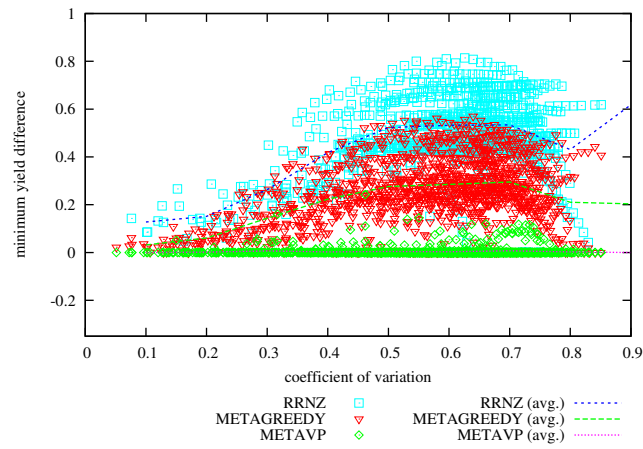
Figure 12: Difference in Achieved Minimum Yield from METAHVP vs Coefficient of Variation on problem instances with 64 hosts, 100 services, memory slack = 0.5
