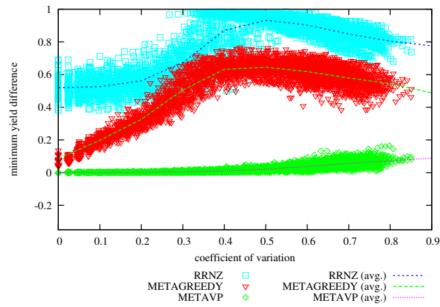
Figure 30: Difference in Achieved Minimum Yield from METAHVP vs Coefficient of Variation on problem instances with 64 hosts, 500 services, memory slack = 0.5
