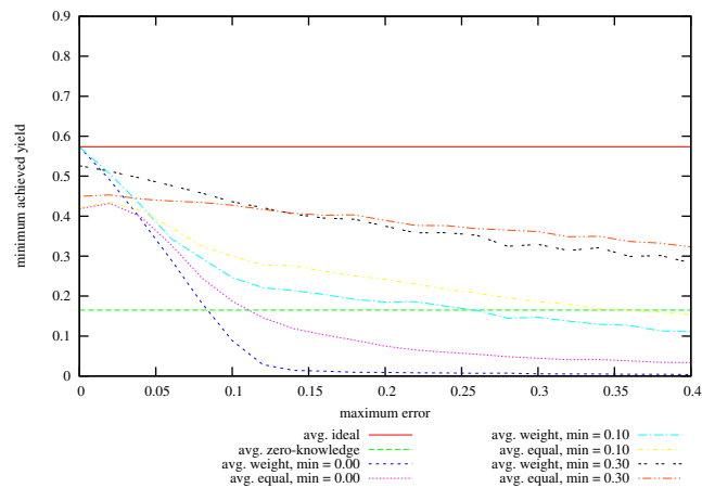
Figure 42: Achieved Minimum Yield from Baseline vs Maximum Specified Error on problem instances with 64 hosts, 100 services, memory slack = 0.8, coefficient of variation = 1.0; values given are averages over successful instances.
