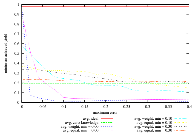
Figure 56: Achieved Minimum Yield from Baseline vs Maximum Specified Error on problem instances with 64 hosts, 500 services, memory slack = 0.4, coefficient of variation = 0.0; values given are averages over successful instances.
