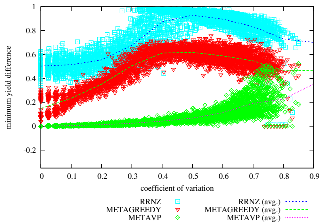
Figure 2: Difference in Achieved Minimum Yield from METAHVP vs Coefficient of Variation on problem instances with 64 hosts, 500 services, memory slack = 0.3
