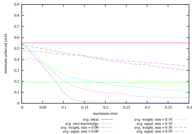
Figure 38: Achieved Minimum Yield from Baseline vs Maximum Specified Error on problem instances with 64 hosts, 100 services, memory slack = 0.6, coefficient of variation = 0.5; values given are averages over successful instances.
