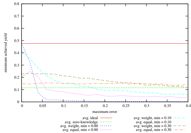
Figure 51: Achieved Minimum Yield from Baseline vs Maximum Specified Error on problem instances with 64 hosts, 250 services, memory slack = 0.2, coefficient of variation = 1.0; values given are averages over successful instances.
