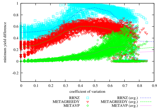
Figure 27: Difference in Achieved Minimum Yield from METAHVP vs Coefficient of Variation on problem instances with 64 hosts, 500 services, memory slack = 0.2
