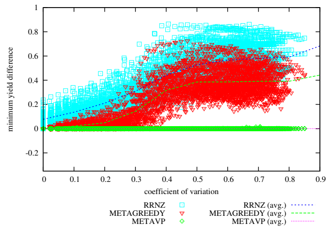
Figure 16: Difference in Achieved Minimum Yield from METAHVP vs Coefficient of Variation on problem instances with 64 hosts, 100 services, memory slack = 0.9
