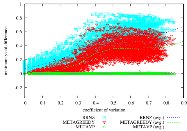
Figure 15: Difference in Achieved Minimum Yield from METAHVP vs Coefficient of Variation on problem instances with 64 hosts, 100 services, memory slack = 0.8
