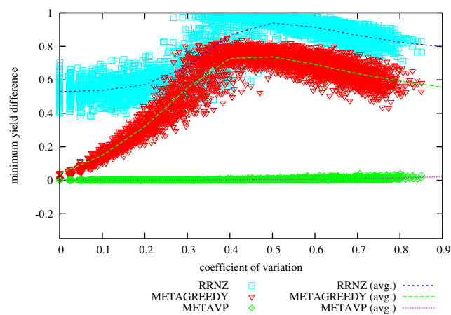
Figure 34: Difference in Achieved Minimum Yield from METAHVP vs Coefficient of Variation on problem instances with 64 hosts, 500 services, memory slack = 0.9
