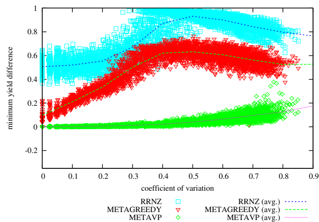
Figure 29: Difference in Achieved Minimum Yield from METAHVP vs Coefficient of Variation on problem instances with 64 hosts, 500 services, memory slack = 0.4
