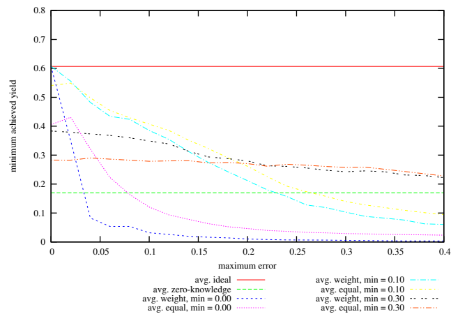
Figure 46: Achieved Minimum Yield from Baseline vs Maximum Specified Error on problem instances with 64 hosts, 250 services, memory slack = 0.8, coefficient of variation = 0.0; values given are averages over successful instances.
