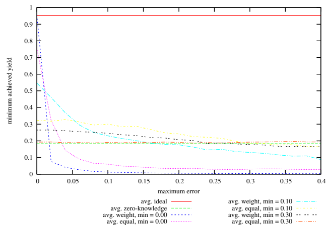
Figure 60: Achieved Minimum Yield from Baseline vs Maximum Specified Error on problem instances with 64 hosts, 500 services, memory slack = 0.4, coefficient of variation = 0.5; values given are averages over successful instances.
