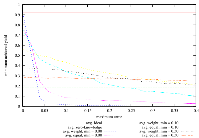
Figure 48: Achieved Minimum Yield from Baseline vs Maximum Specified Error on problem instances with 64 hosts, 250 services, memory slack = 0.4, coefficient of variation = 0.5; values given are averages over successful instances.
