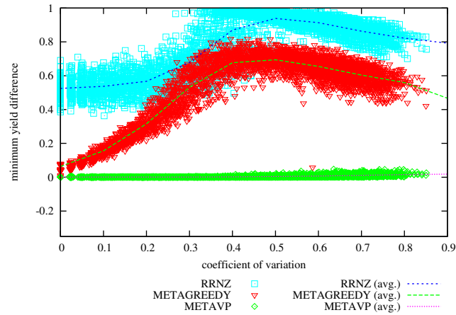
Figure 33: Difference in Achieved Minimum Yield from METAHVP vs Coefficient of Variation on problem instances with 64 hosts, 500 services, memory slack = 0.8
