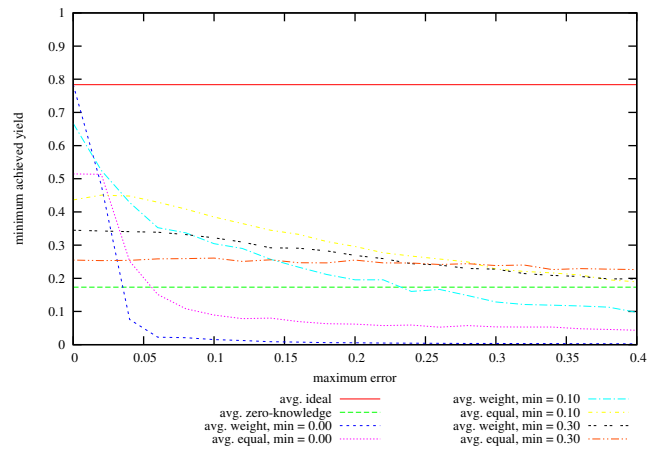
Figure 47: Achieved Minimum Yield from Baseline vs Maximum Specified Error on problem instances with 64 hosts, 250 services, memory slack = 0.2, coefficient of variation = 0.5; values given are averages over successful instances.
