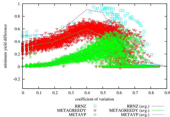
Figure 26: Difference in Achieved Minimum Yield from METAHVP vs Coefficient of Variation on problem instances with 64 hosts, 500 services, memory slack = 0.1
