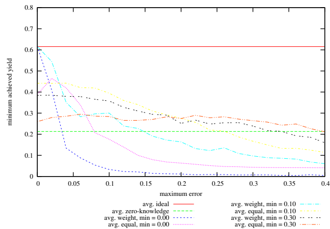
Figure 44: Achieved Minimum Yield from Baseline vs Maximum Specified Error on problem instances with 64 hosts, 250 services, memory slack = 0.4, coefficient of variation = 0.0; values given are averages over successful instances.
