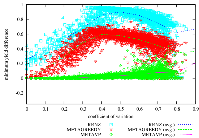
Figure 19: Difference in Achieved Minimum Yield from METAHVP vs Coefficient of Variation on problem instances with 64 hosts, 250 services, memory slack = 0.3
