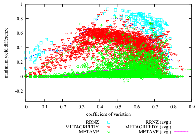
Figure 18: Difference in Achieved Minimum Yield from METAHVP vs Coefficient of Variation on problem instances with 64 hosts, 250 services, memory slack = 0.2
