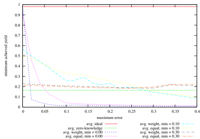
Figure 58: Achieved Minimum Yield from Baseline vs Maximum Specified Error on problem instances with 64 hosts, 500 services, memory slack = 0.8, coefficient of variation = 0.0; values given are averages over successful instances.
