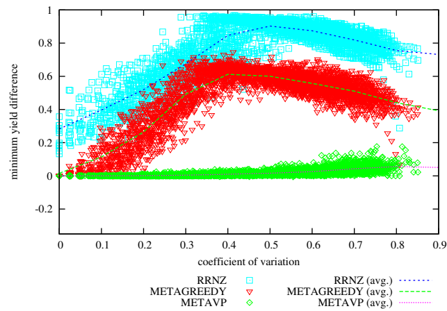
Figure 20: Difference in Achieved Minimum Yield from METAHVP vs Coefficient of Variation on problem instances with 64 hosts, 250 services, memory slack = 0.4
