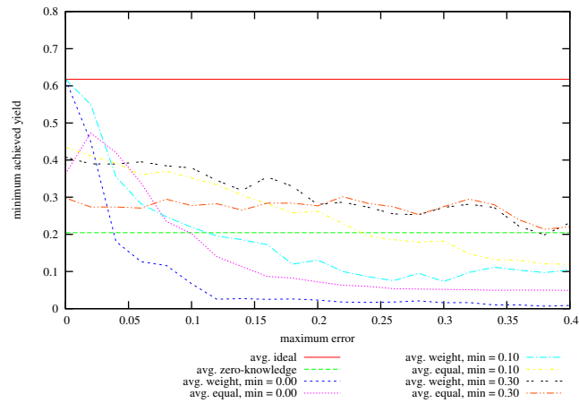
Figure 43: Achieved Minimum Yield from Baseline vs Maximum Specified Error on problem instances with 64 hosts, 250 services, memory slack = 0.2, coefficient of variation = 0.0; values given are averages over successful instances.
