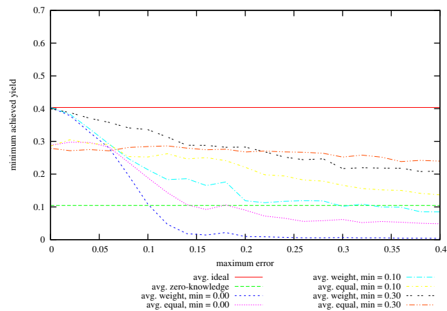
Figure 40: Achieved Minimum Yield from Baseline vs Maximum Specified Error on problem instances with 64 hosts, 100 services, memory slack = 0.4, coefficient of variation = 1.0; values given are averages over successful instances.
