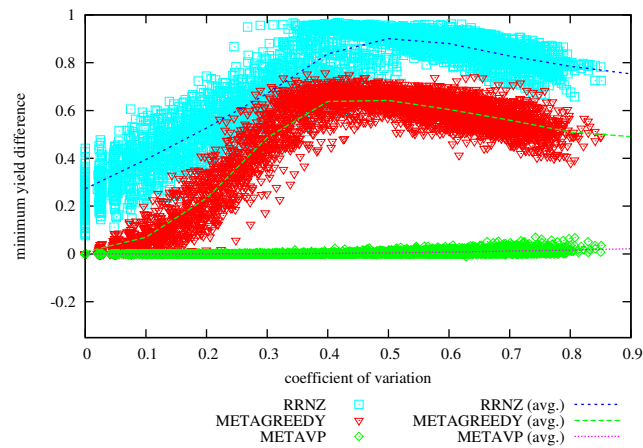
Figure 22: Difference in Achieved Minimum Yield from METAHVP vs Coefficient of Variation on problem instances with 64 hosts, 250 services, memory slack = 0.6
