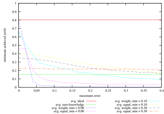
Figure 53: Achieved Minimum Yield from Baseline vs Maximum Specified Error on problem instances with 64 hosts, 250 services, memory slack = 0.6, coefficient of variation = 1.0; values given are averages over successful instances.
