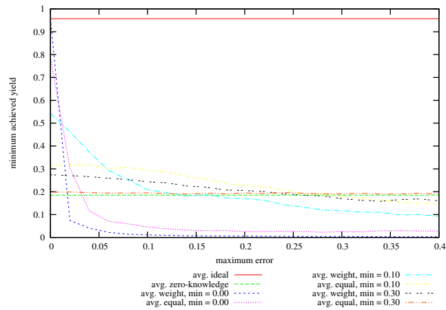
Figure 61: Achieved Minimum Yield from Baseline vs Maximum Specified Error on problem instances with 64 hosts, 500 services, memory slack = 0.6, coefficient of variation = 0.5; values given are averages over successful instances.
