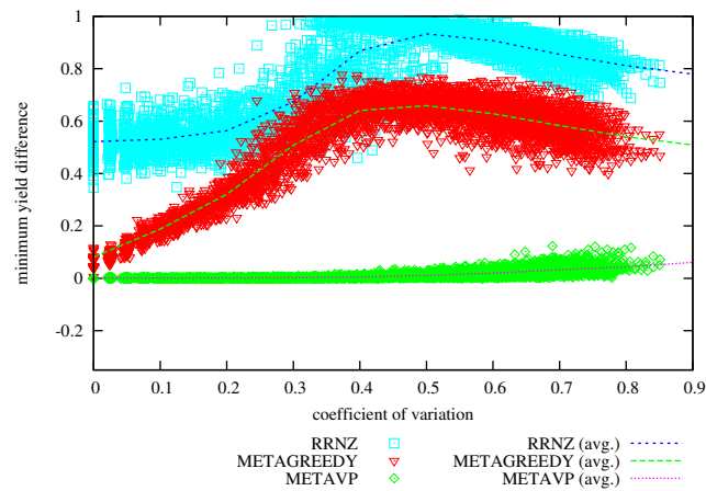
Figure 31: Difference in Achieved Minimum Yield from METAHVP vs Coefficient of Variation on problem instances with 64 hosts, 500 services, memory slack = 0.6
