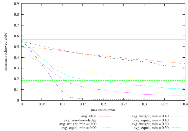
Figure 39: Achieved Minimum Yield from Baseline vs Maximum Specified Error on problem instances with 64 hosts, 100 services, memory slack = 0.8, coefficient of variation = 0.5; values given are averages over successful instances.
