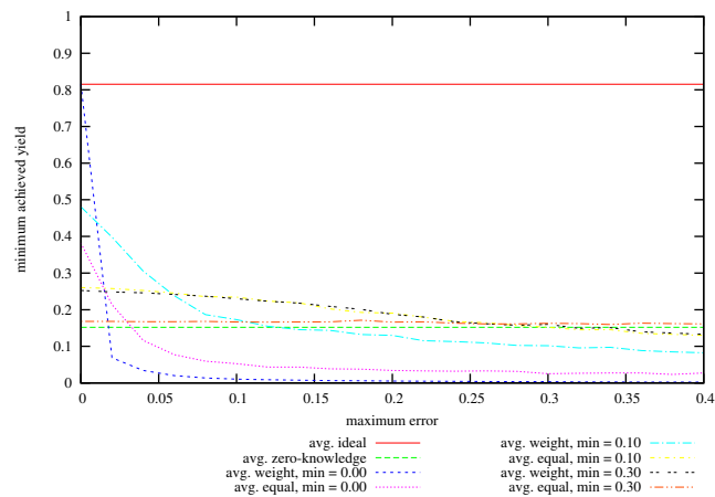
Figure 64: Achieved Minimum Yield from Baseline vs Maximum Specified Error on problem instances with 64 hosts, 500 services, memory slack = 0.4, coefficient of variation = 1.0; values given are averages over successful instances.
