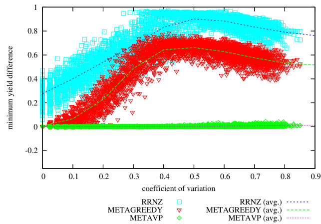
Figure 23: Difference in Achieved Minimum Yield from METAHVP vs Coefficient of Variation on problem instances with 64 hosts, 250 services, memory slack = 0.7
