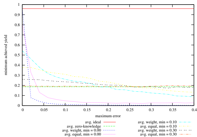
Figure 62: Achieved Minimum Yield from Baseline vs Maximum Specified Error on problem instances with 64 hosts, 500 services, memory slack = 0.8, coefficient of variation = 0.5; values given are averages over successful instances.
