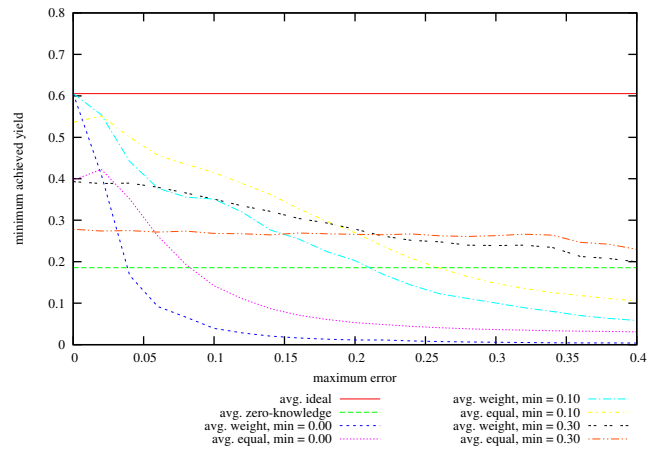
Figure 45: Achieved Minimum Yield from Baseline vs Maximum Specified Error on problem instances with 64 hosts, 250 services, memory slack = 0.6, coefficient of variation = 0.0; values given are averages over successful instances.
