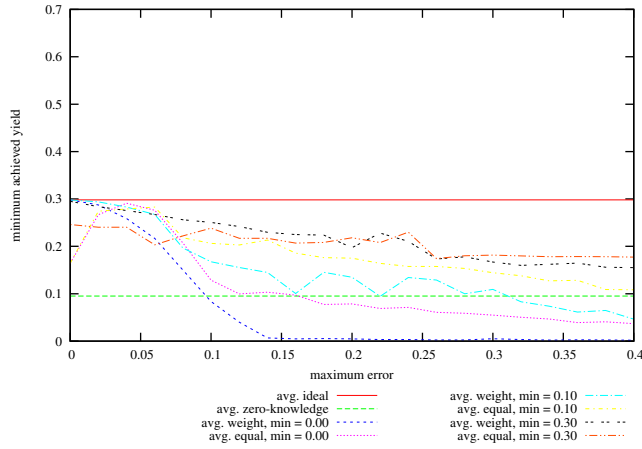
Figure 5: Achieved Minimum Yield from Baseline vs Maximum Specified Error on problem instances with 64 hosts, 100 services, memory slack = 0.4, coefficient of variation = 0.5; values given are averages over successful instances.
