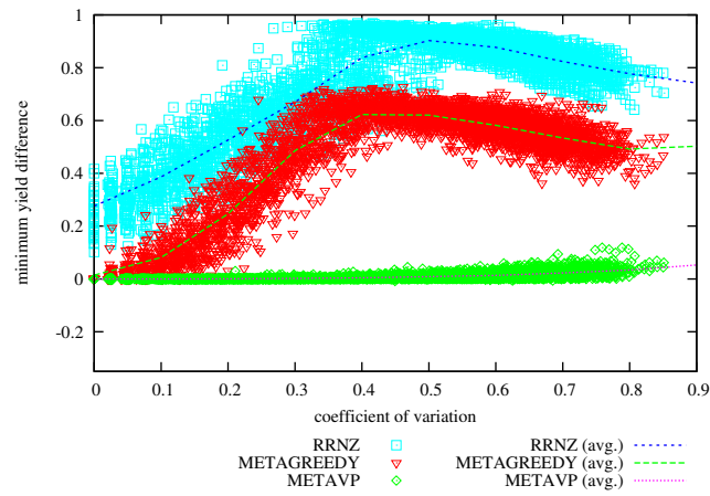
Figure 21: Difference in Achieved Minimum Yield from METAHVP vs Coefficient of Variation on problem instances with 64 hosts, 250 services, memory slack = 0.5
