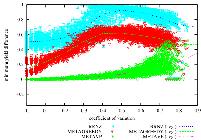
Figure 28: Difference in Achieved Minimum Yield from METAHVP vs Coefficient of Variation on problem instances with 64 hosts, 500 services, memory slack = 0.3
