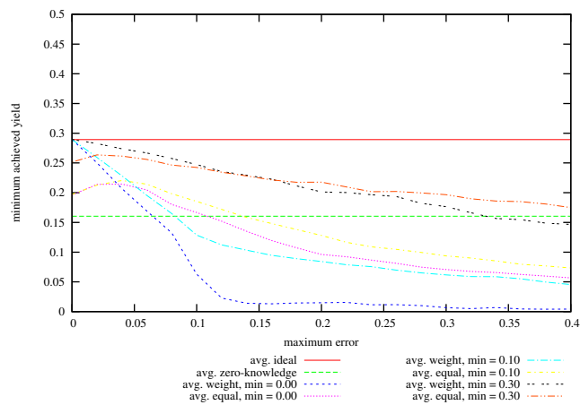
Figure 36: Achieved Minimum Yield from Baseline vs Maximum Specified Error on problem instances with 64 hosts, 100 services, memory slack = 0.8, coefficient of variation = 0.0; values given are averages over successful instances.
