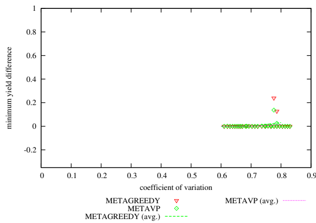
Figure 10: Difference in Achieved Minimum Yield from METAHVP vs Coefficient of Variation on problem instances with 64 hosts, 100 services, memory slack = 0.3
