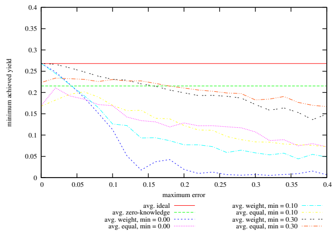
Figure 35: Achieved Minimum Yield from Baseline vs Maximum Specified Error on problem instances with 64 hosts, 100 services, memory slack = 0.6, coefficient of variation = 0.0; values given are averages over successful instances.
