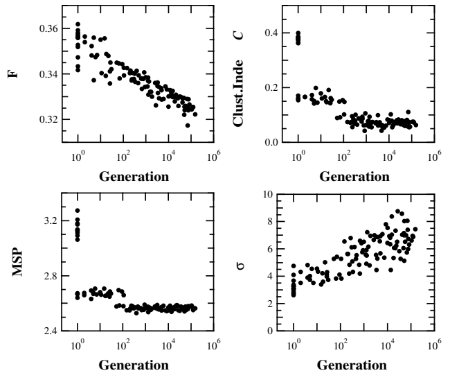
Figure 6: Time courses of the main network statistics during artificial evolution. Each time a mutation gives rise to a topology with a better fitness than the best one in the current population, its fitness (A), average mean shortest path (B), average clustering index \langle C \rangle (C) and the standard deviation of its connectivity distribution \sigma_k (D) are plotted against the current generation number. Each panel groups the results of 9 evolution runs. Parameters: \eta(0) = 0.35 , fitness estimated as an average over 5 independent runs of 10,000 learning iterations with 2,000 examples from the training set and 5,000 examples from the test set.
