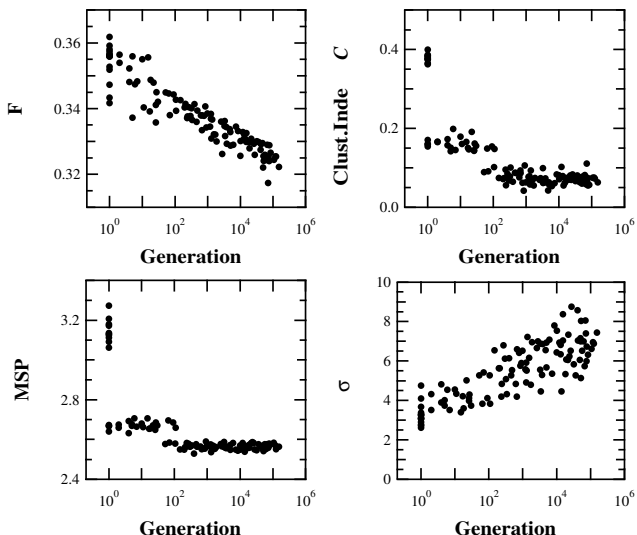
Figure 6: Time courses of the main network statistics during artificial evolution. Each time a mutation gives rise to a topology with a better fitness than the best one in the current population, its fitness (A), average mean shortest path (B), average clustering index \langle C \rangle (C) and the standard deviation of its connectivity distribution \sigma_k (D) are plotted against the current generation number. Each panel groups the results of 9 evolution runs. Parameters: \eta(0) = 0.35 , fitness estimated as an average over 5 independent runs of 10,000 learning iterations with 2,000 examples from the training set and 5,000 examples from the test set.
