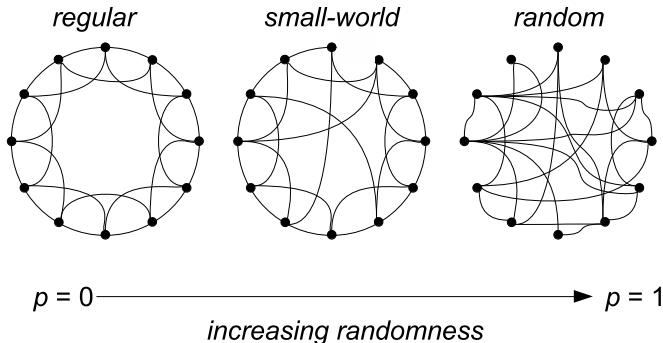
Figure 1: Small-world networks according to Watts and Strogatz. Starting with a regular ring network ( p = 0 , left), each link is rewired to a randomly-chosen destination node with probability p . When p = 1 (right), the network is a random one. At small-to-intermediate p values (depending on the network size), the network displays small-world properties (center). Adapted from [20].
