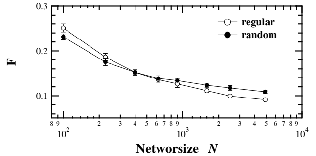
Figure 5: Performance F vs number of neurons N after 10^6 learning steps for regular (rewiring probability p = 0 , white circles) or random ( p = 1 , black circles) topologies. Each point is an average over 11 random initial weight and topology realizations. Vertical bars are standard deviations. Stars indicate statistically significant differences (unpaired t -test, p < 0.010 ). Other parameters as in Figure 4-A.
