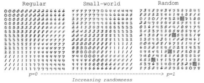
Figure 3: Results of the learning phase using the three topology classes shown in Figure 2. The weight vector \mathbf{w}_i of each neuron i is represented as a 28 \times 28 image, centered on the neuron position in the 2d grid. For the random network, some neurons are disconnected from the network, and thus do not learn from the examples during the learning phase. Their weight vectors are thus kept random, yielding the random images on the figure.
