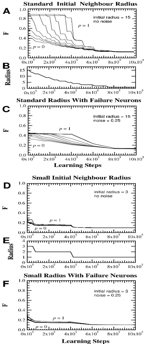
Figure 4: Evolution of the performance F during learning for SOMs on complex neighborhood networks. Neighborhood networks are constructed positioning neurons on a square grid, and linking each neuron to its 8-nearest neighbors on the grid (Moore neighborhood). Each link is then rewired to a (uniformly) randomly-chosen destination neuron with probability p = 0, 0.002, 0.004, 0.008, 0.016, 0.032, 0.064, 0.256, 1.000 (from bottom to top). Panels A, C, D and F show the evolution of the fitness F for different values initial radius and noise levels (as indicated on each panels). Panels B and E display the evolution of the neighborhood radius. Other parameters: map size N = 1024 neurons, initial learning rate \eta(0) = 0.080 , training and test sets of 30,000 and 10,000 examples, respectively.
