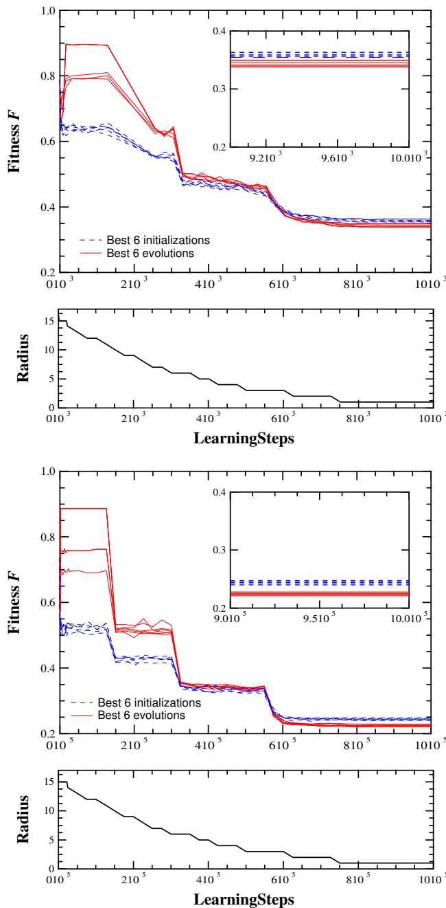
Figure 7: Evolution of the fitness during learning of the 6 best networks from the initialization phase (dashed lines) and the 6 best networks obtained after evolution (full lines). The learning protocol consisted of 10^4 (upper panels) or 10^6 (lower panels) learning steps. The insets show magnified views of the results at the end of the learning phase. The evolution of the neighborhood radius is also given in each case for comparison purposes. Each curve is an average over 11 initial realizations of the neuron weights.
