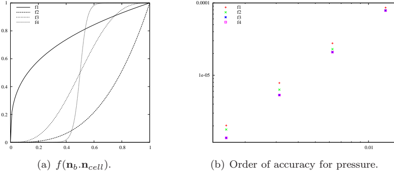
Figure 5: Comparison of the L_\infty error for pressure for different choices of f(\mathbf{n}_b \cdot \mathbf{n}_{cell}) .
