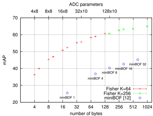
Fig. 5. mAP for a search on Holidays with varying ADC quantization parameters (number of bytes). Results of [12] are reported with circles for reference.
