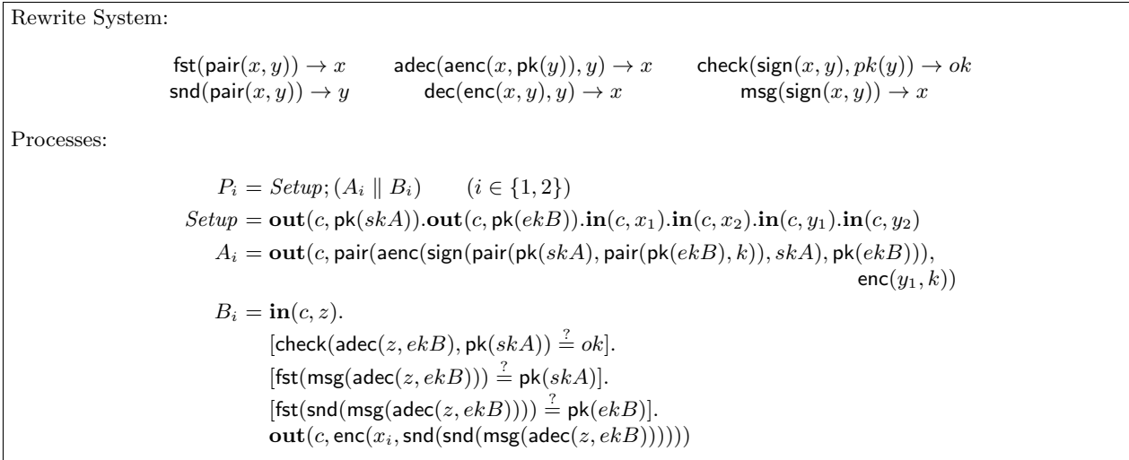
Fig. 6: Formal description of the variant protocol by Blanchet
