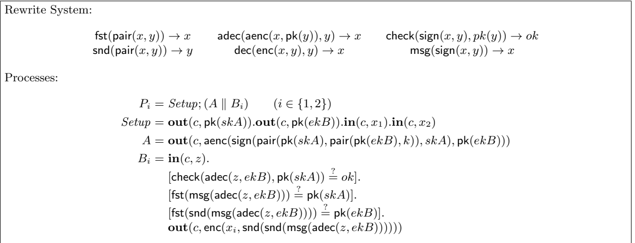
Fig. 5: Formal description of the protocol by Blanchet
