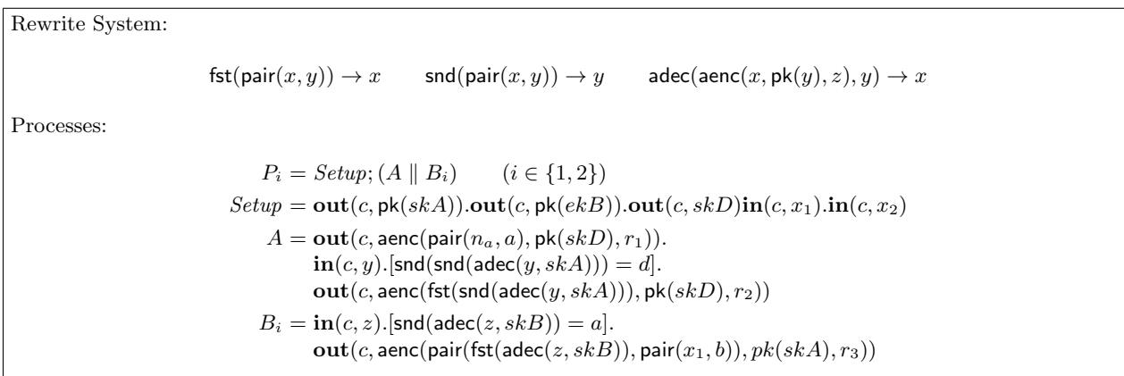
Fig. 7: Formal description of the NSL protocol
