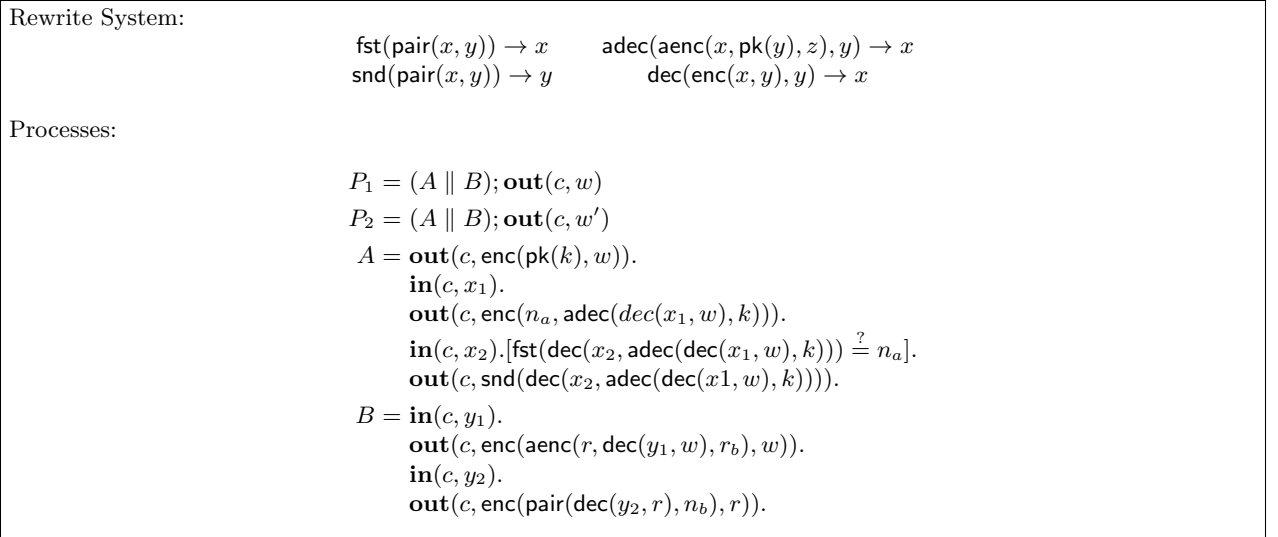
Fig. 8: Formal description of the EKE protocol
