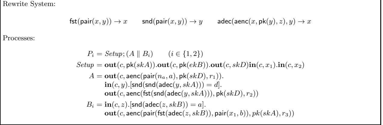
Fig. 7: Formal description of the NSL protocol
