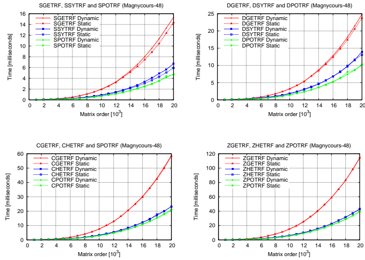
Figure 7: Execution time of xPOTRF, xSYTRF / xHETRF and xGETRF; dynamic (solid line) and static (dashed line) scheduling.
