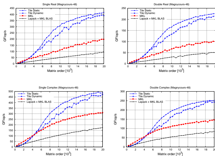
Figure 6: Performance of SRBT-LDL T against MKL and LAPACK .
