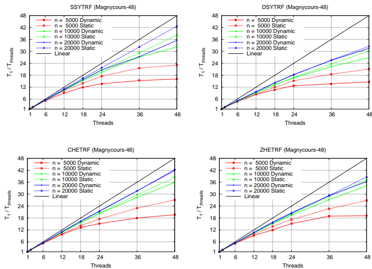
Figure 8: xSYTRF / xHETRF scalability; dynamic (solid line) and static (dashed line) scheduling.
