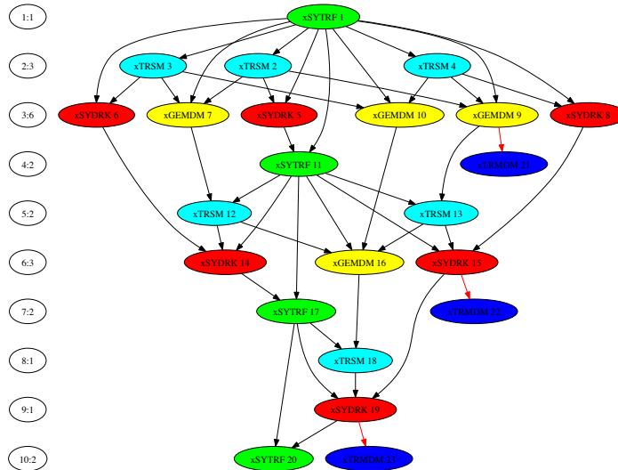
Figure 4: DSYTRF DAG; NT = 4 .
