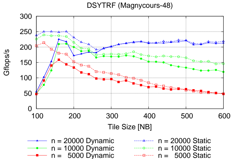
Figure 9: Tile-size performance of tiled DSYTRF, dynamic (solid line) and static (dashed line) scheduling ( IB = 125 ).
