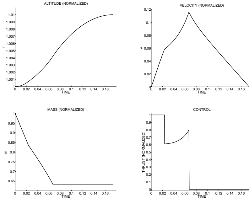
Figure 3: Goddard Problem
