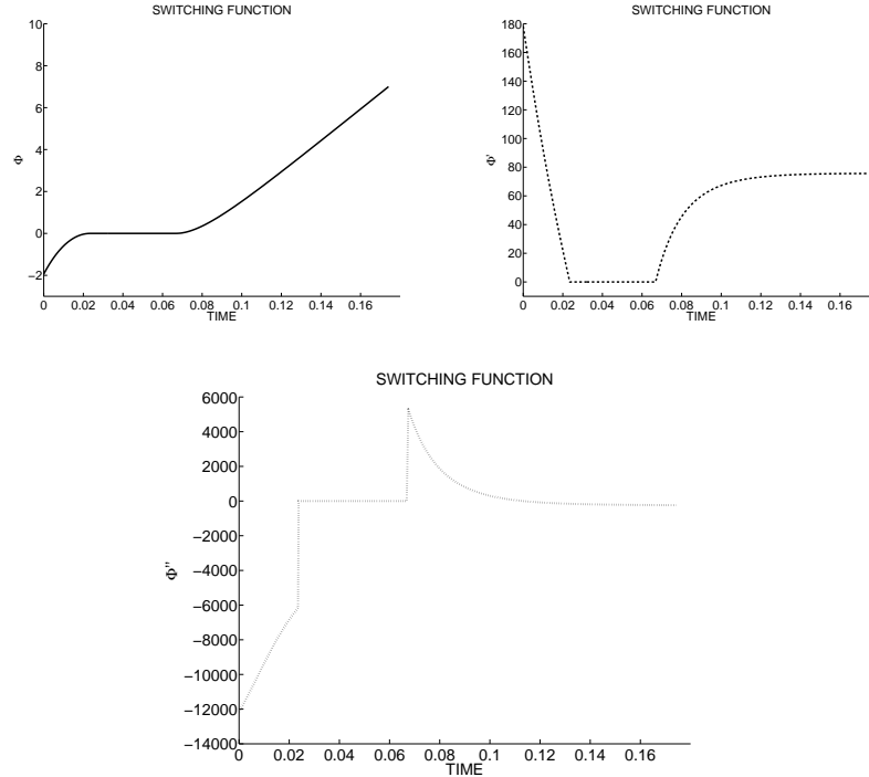
Figure 4: Goddard Problem
