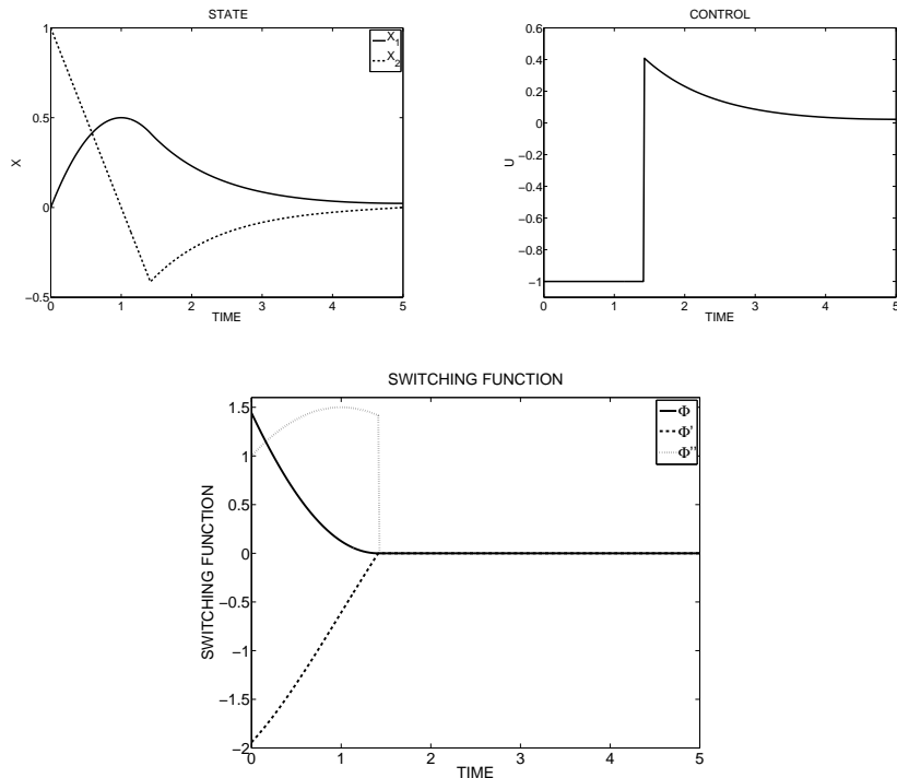
Figure 2: Regulator Problem
