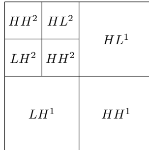
Figure 5: Wavelet transform for a scale 2.
