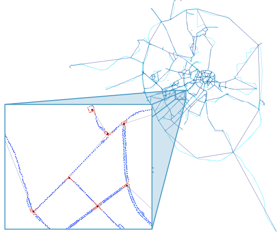
Figure 3: GPS traces: the input neighborhood graph is shown in cyan, the points marked as belonging to a branch are shown in red, and the points marked as belonging to an edge are shown in blue. The reconstructed graph is shown in dark blue.
