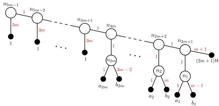
Figure 5: Instance \mathcal{I}_6 .
