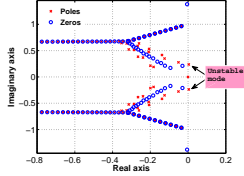
Figure 3. Poles and zeros of the reduced linearized system for Re = 10\,000 , \alpha_n = 1 .
