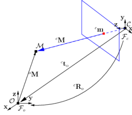
Figure 5. Perspective projection of a flow particle.
