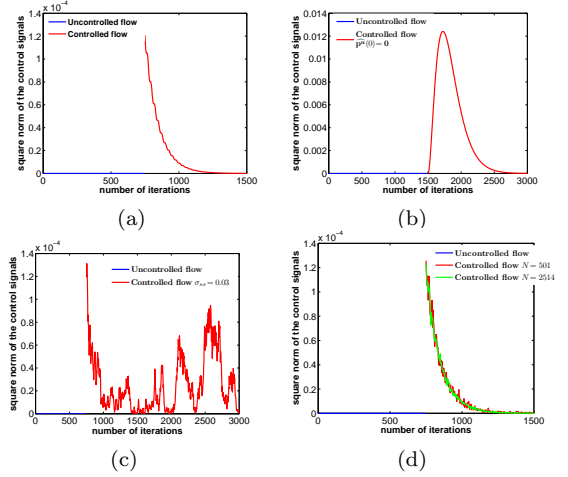
Fig. 7. Comparison LQG and the vision-based control approaches: (a) ideal case, (b) initialization error in the LQG regulator, (c) measurements noise in the LQG regulator, (d) measurements noise in the vision-based control.
