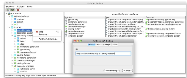
Figure 2. FraSCAti Explorer.
