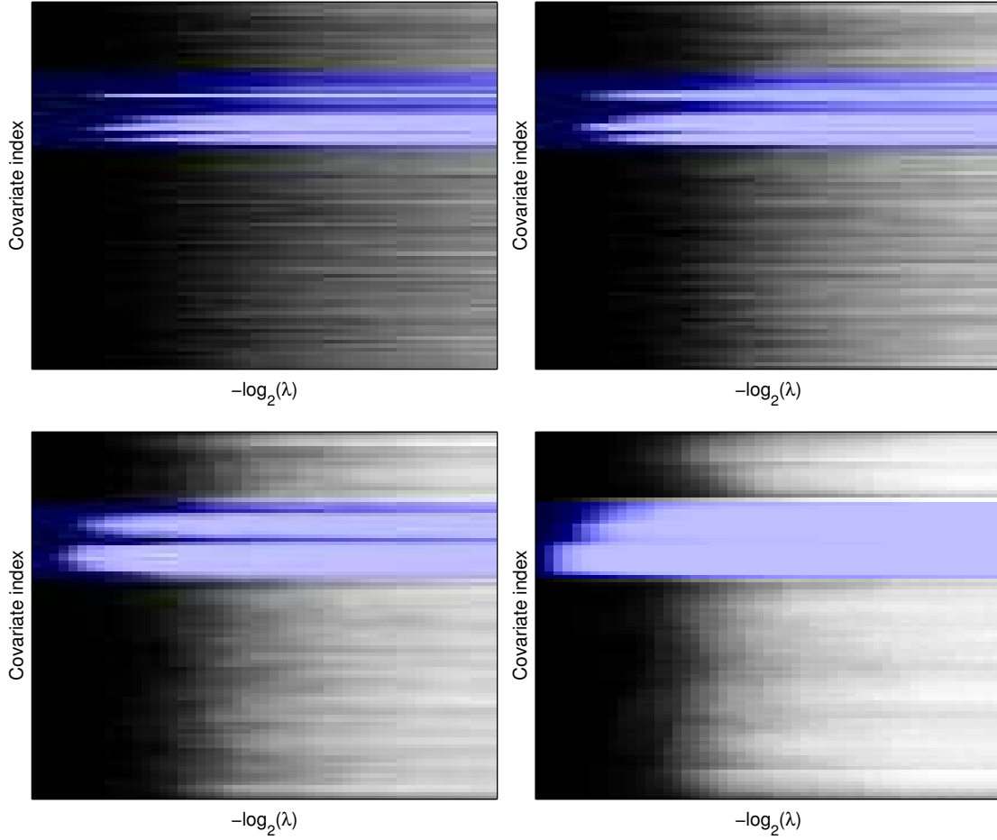
Figure 8: Variable selection frequency with \Omega_{\mathcal{G}}^{\mathcal{G}} using the chains of length k (left) as groups, for k = 1 (Lasso), 2, 4, 8. For each variable index (on the y-axis), its frequency of selection is represented in levels of gray as a function of the regularization parameter \lambda (on the x-axis), both for the Lasso penalty and \Omega_{\mathcal{G}}^{\mathcal{G}} . The transparent blue band superimposed indicates the covariates that belong to the support.
