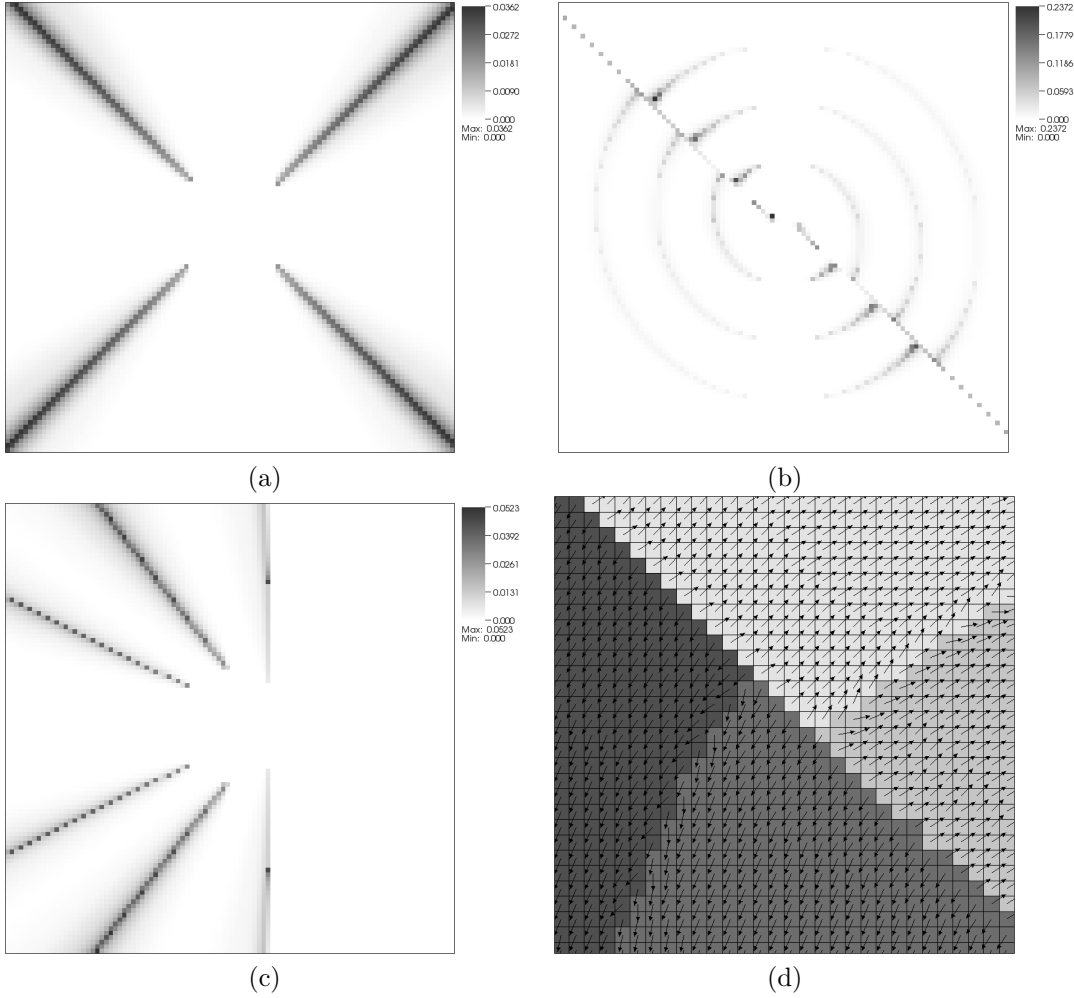
FIG. 4.2. Patchy error E_P , \tilde{N} = 50 \rightarrow N = 100 for (a) Eikonal, (b) Fan, (c) Zermelo. In (d) it is shown a detail of the patchy decomposition for the Fan dynamics, together with the optimal vector field f(x, a^*) computed by means of the final patchy solution.
