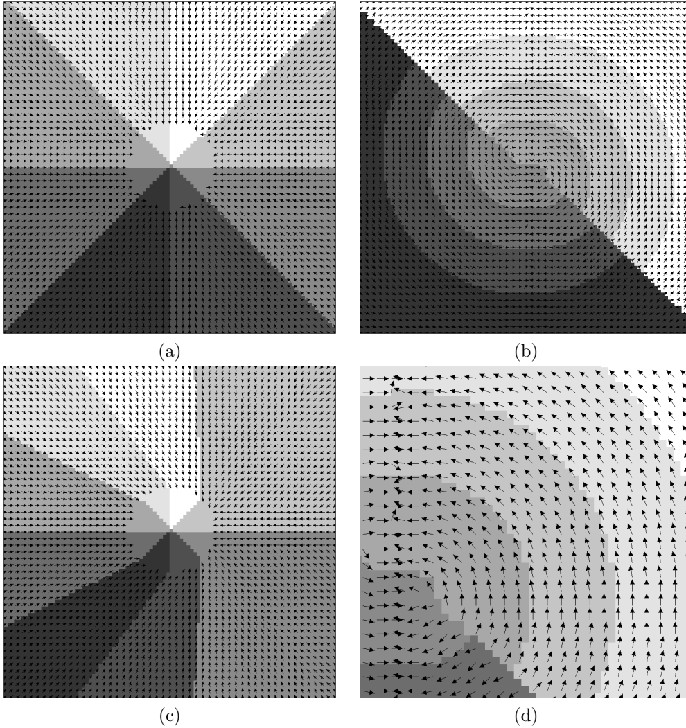
FIG. 4.1. Patchy decompositions with R = 8 , N_c = 32 , \tilde{N} = 50 and N = 100 . Only few arrows are shown for clarity of visualization. (a) Eikonal, (b) Fan, (c) Zermelo, (d) a detail of (b).
