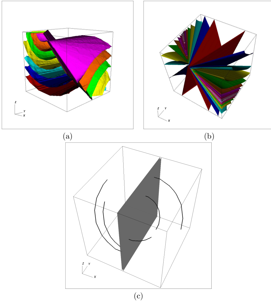
FIG. 6.2. (a) Decomposition with 8 patches, (b) level sets of the solution, and (c) some optimal trajectories to the target
