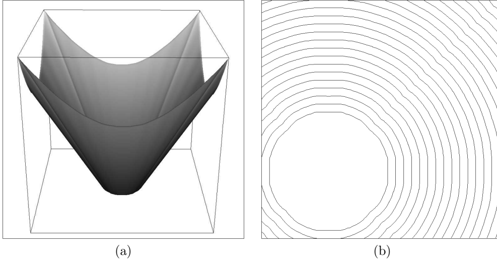
FIG. 4.3. Patchy solution for the dynamics Eikonal. (a) Value function and (b) a detail of its level sets. Small hollows are visible in correspondence of the lines \{x = y\} and \{x = -y\} as in Fig. 4.2-(a).
