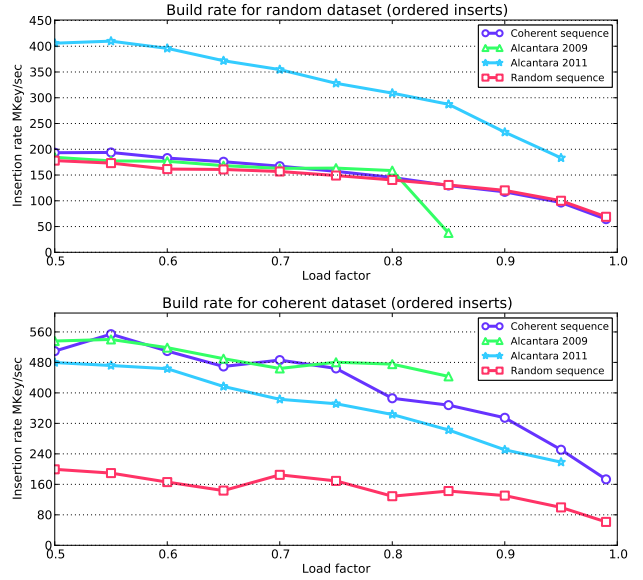
Figure 6: Construction times for h_{rand} and h_{coh} and earlier schemes. Times are averaged over several runs. Top: 1M random keys are inserted, taken from a universe of size 8K \times 8K . Bottom: Timings for the fish image: 20.5M are defined in a universe of size 8K \times 8K .
