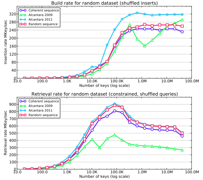
Figure 5: Insertion rates (top) and retrieval rates (bottom) for h_{rand} and h_{coh} , and earlier schemes, for increasingly larger input, under 0.8 load factor. Timings are averaged over several runs. Please refer to the text for details on these data sets.
