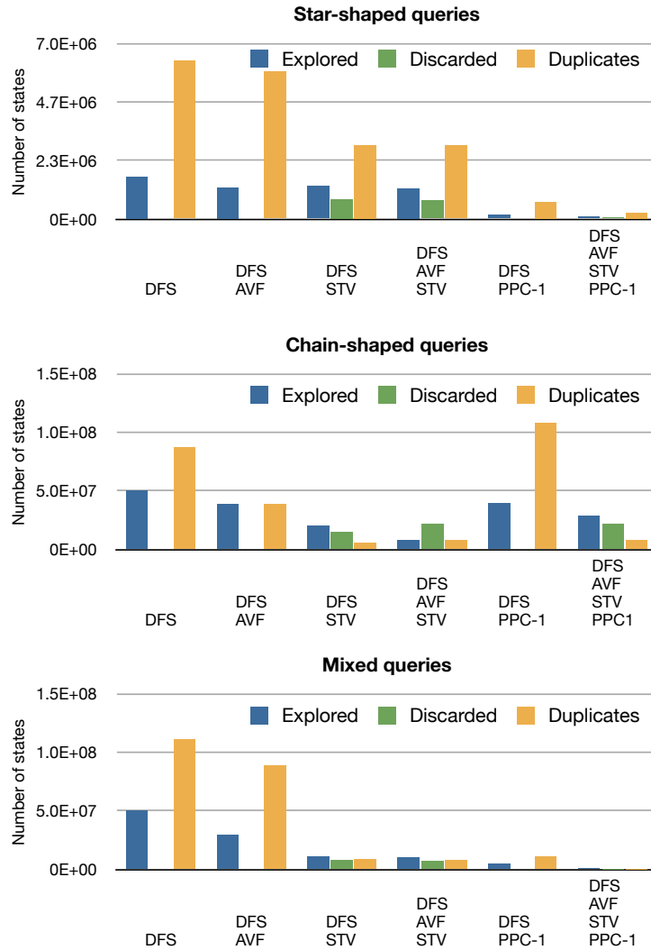
Figure 6: Impact of heuristics on the DFS strategy for star, chain and mixed query workloads.
