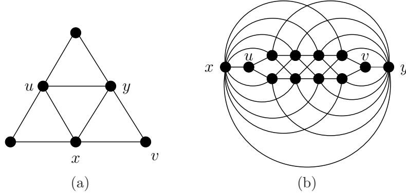
FIGURE 3. Two graphs in (a) \mathcal{CWW}(k) \setminus \mathcal{CWF}(k) , k \geq 2 and (b) \mathcal{CWW}(4) \setminus \mathcal{CWW}(5) .
