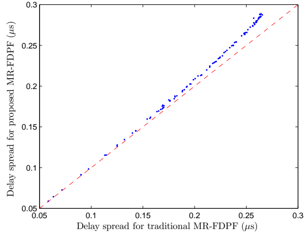
Figure 6: CITI. Estimated delay spread N = 2 ( \nu_0 = 2.35 GHz).
