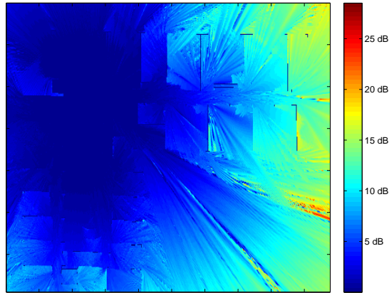
Figure 7: CITI. Spatial distribution of the approximation error at \nu = 2.347 GHz and N = 2 ( \nu_0 = 2.35 GHz).
