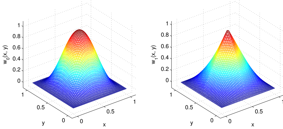
Figure 9: Initial conditions in (53)
