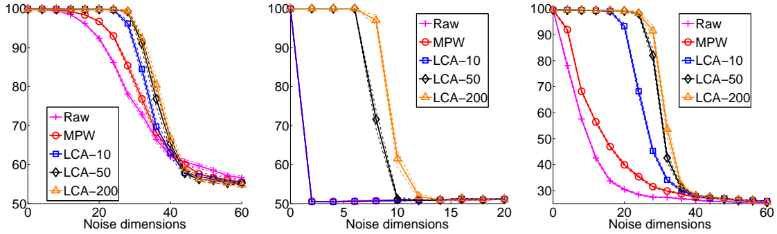
Figure 4: Average clustering accuracy (100% = perfect clustering, chance is 50% for the first two datasets and 20% for the last one) on 100 runs for varying number of dimensions of noise added and varying number of EM iterations in the LCA algorithm (MPW = one iteration). The error bars represent one standard error. Left: mixture of isotropic Gaussians presented in Fig. (2) (left). Centre: two concentric circles presented in Fig. (2) (centre). Right: mixture of five Gaussians presented in Fig. (2) (right). Figure best seen in colour.
