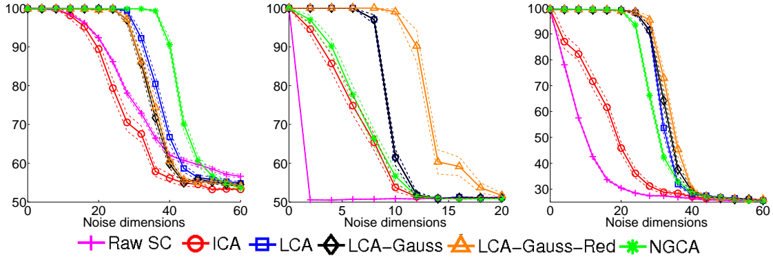
Figure 3: Average clustering accuracy (100% = perfect clustering, chance is 50% for the first two datasets and 20% for the last one) on 100 runs for varying number of dimensions of noise added. The error bars represent one standard error. Left: mixture of isotropic Gaussians presented in Fig. (2) (left). Centre: two concentric circles presented in Fig. (2) (centre). Right: mixture of five Gaussians presented in Fig. (2) (right). Figure best seen in colour.
