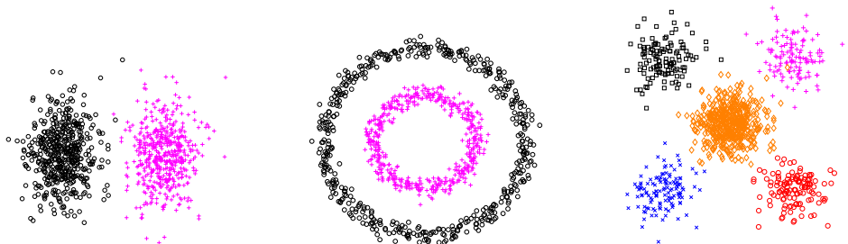
Figure 2: Noise-free data used to assess the robustness of K -means to noise. Left: mixture of two isotropic Gaussians of unit variance and means [-3, 0]^T and [3, 0]^T . Centre: two concentric circles with radii 1 and 2, with added isotropic Gaussian noise of standard deviation .1. Right: mixture of five Gaussians. The centre cluster contains four times as many datapoints as the other ones.
