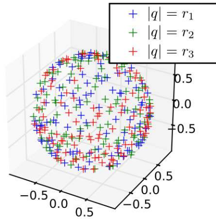
Fig. 2 - 300 points optimized for 3 shells, projected on the unit sphere.
