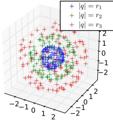
Fig. 1 - 300 points optimized for 3 shells
