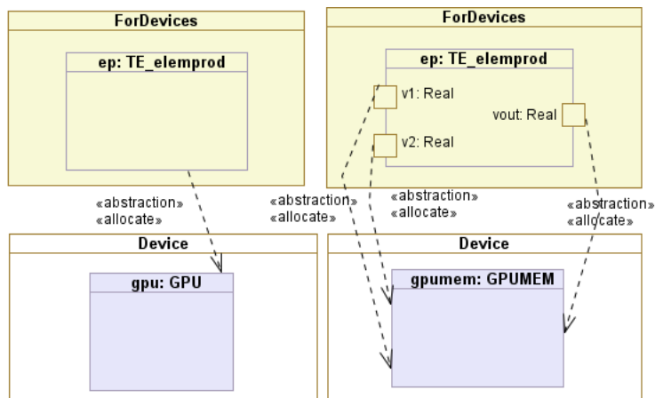
Figure 9: Vector Product Application Model
