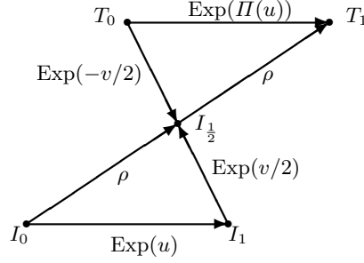
Fig. 1: Schild's Ladder parallelogram with the one parameter subgroups. The transport \text{Exp}(II(u)) is the deformation \text{Exp}(v/2) \circ \text{Exp}(u) \circ \text{Exp}(-v/2)
