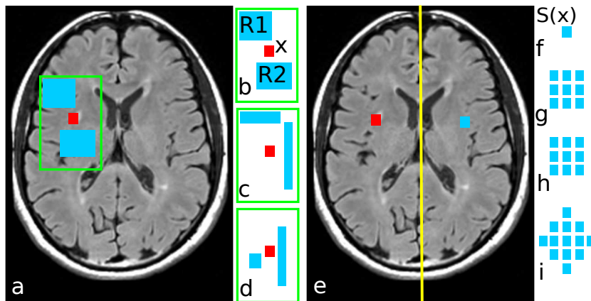
Figure 4: 2D view of context-rich features. (a) A context-rich feature depicting two regions R_1 and R_2 with constant offset relatively to \mathbf{x} . (b-d) Three examples of randomly sampled features in an extended neighborhood. (e) The symmetric feature with respect to the mid-sagittal plane. (f) The hard symmetric constraint. (g-i) The soft symmetry feature considering neighboring voxels in a sphere of increasing radius. See text for details.
