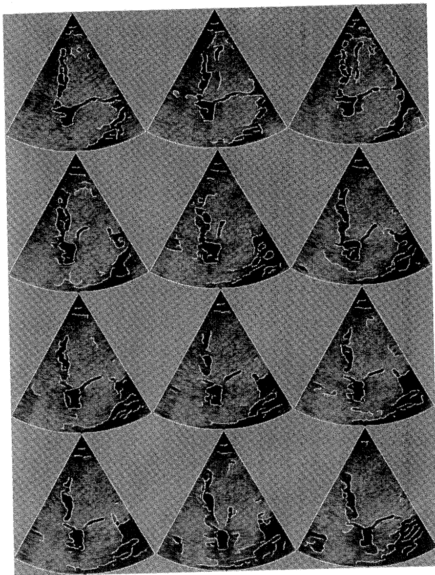
Figure 17.8 Edges.
