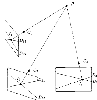
Fig. 1. Geometric constraints of trinocular stereo vision.
