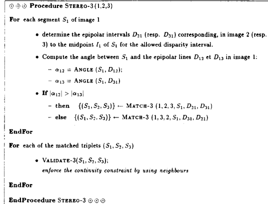
Fig. 12. Trinocular stereo vision algorithm.
